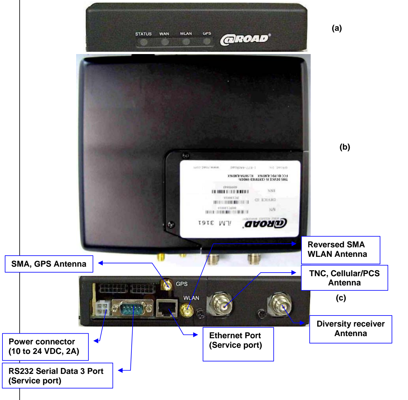
iLM316X-W external (a) Front view, (b) top view, (c) Rear view
