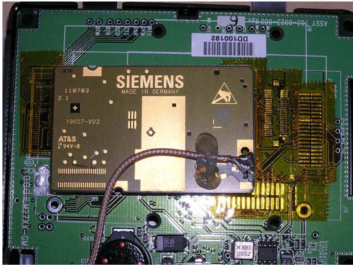
PCB Top view showing GSM Module
