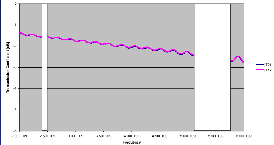
Transmission Loss / 458 mm
