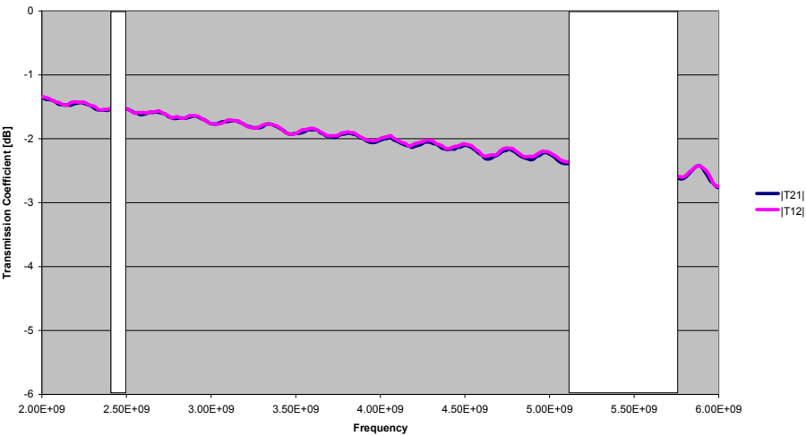
Transmission Loss / 458 mm
