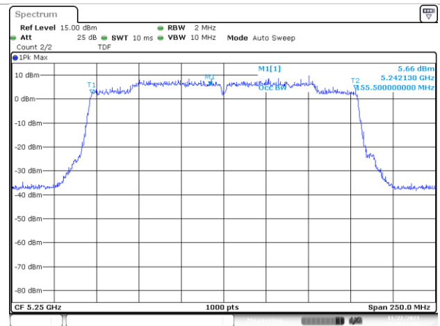
MIMO A-802.11ax/be-160MHz-50-5250-MCS0 99%
