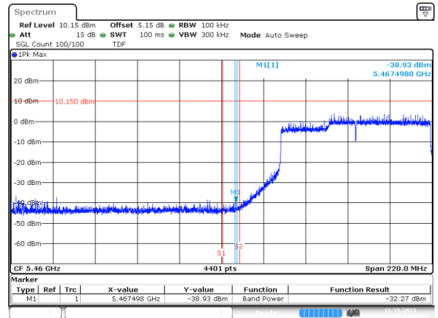
BE-NR-LOW, SISO-A, 802.11ax/be160-MCS0, Ch114
