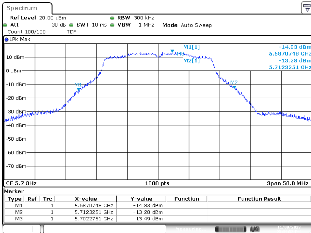
SISO A-802.11n20-CH140-5700MHz-HT0
