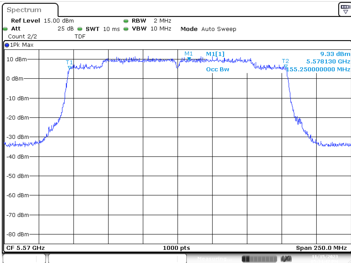
MIMO A-802.11ax/be160-CH114-5570MHz-MCS0
