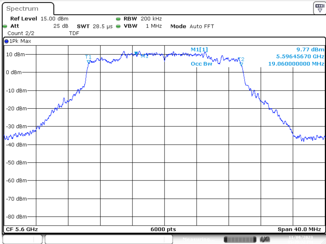
SISO A-802.11ax/be20-CH120-5600MHz-MCS0
