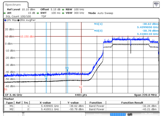
BE-R-LOW, SISO-A, 802.11ax/be80-MCS0, Ch106
