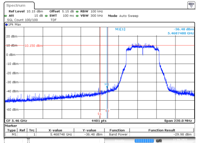
BE-NR-LOW, SISO-A, 802.11ax/be40-MCS0, Ch102
