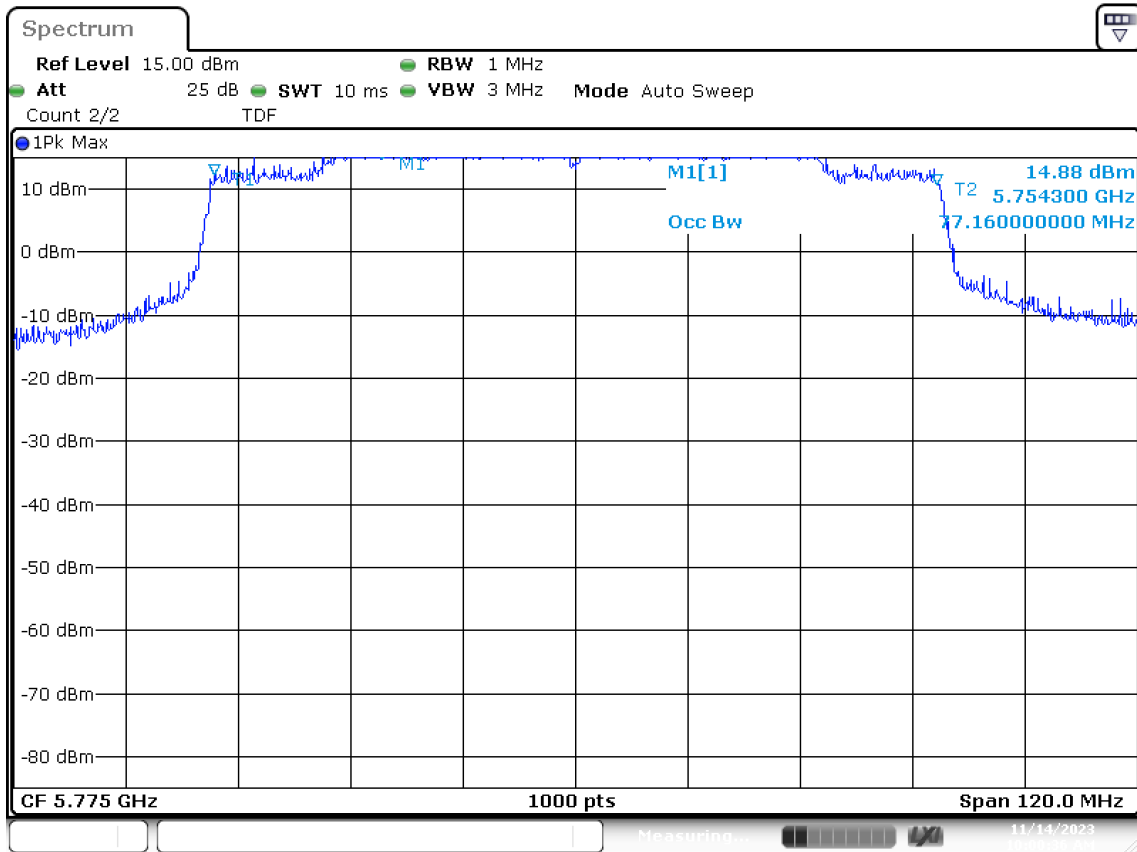
SISO B-802.11ax/be80-CH155-5775MHz-MCS0
