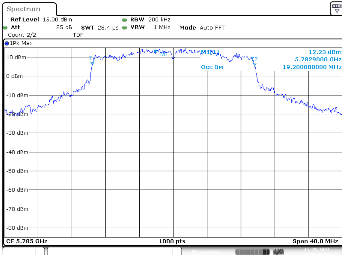
SISO A-802.11ax/be20-CH157-5785MHz-MCS0
