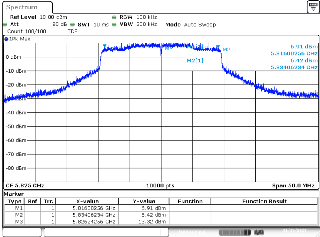
SISO A-802.11ax/be20-CH165-5825MHz-MCS0
