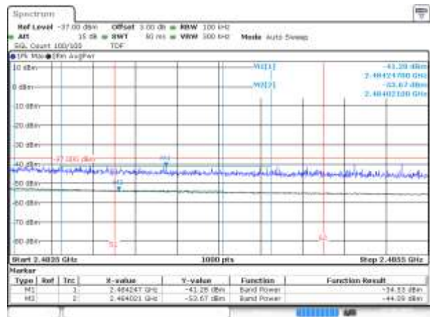
BE-R-HIGH-2MHz, SISO-A, 802.11ax20-MCS0, Ch11
