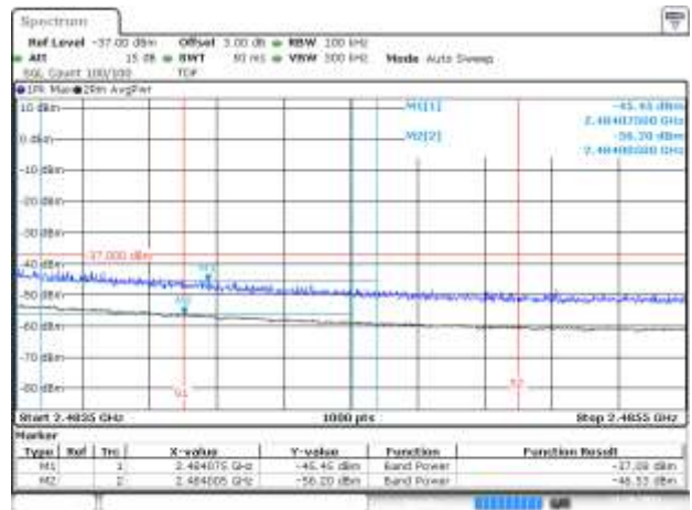
BE-R-HIGH-2MHz, MIMO-A, 802.11ax20-MCS0, Ch12
