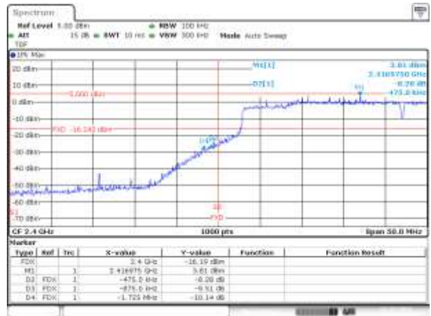
BE-NR, MIMO-B, 802.11ax40-MCS0, Ch3
