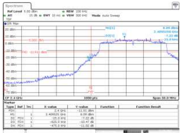
BE-NR, MIMO-A, 802.11ax20-MCS0, Ch1
