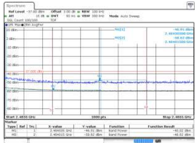
BE-R-HIGH-2MHz, MIMO-B, 802.11ax40-MCS0, Ch11
