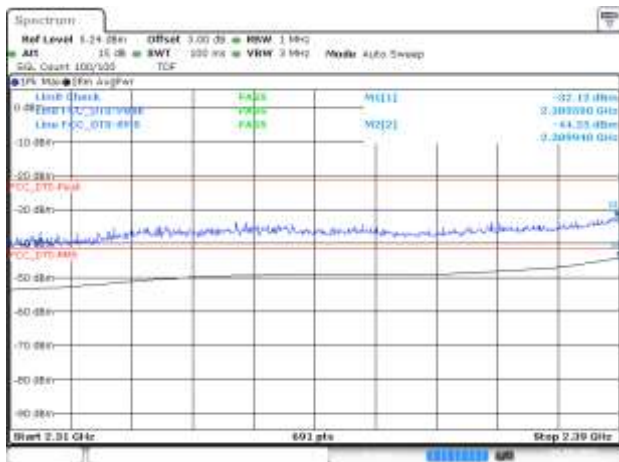
BE-R-LOW, SISO-B, 802.11ax40-MCS0, Ch3
