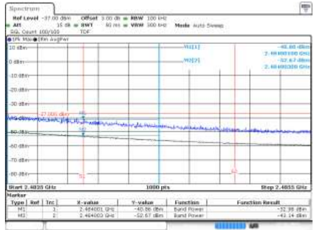
BE-R-HIGH-2MHz, SISO-B, 802.11ax20-MCS0, Ch12
