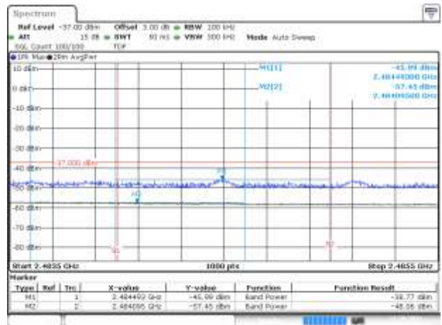
BE-R-HIGH-2MHz, MIMO-A, 802.11ax40-MCS0, Ch9
