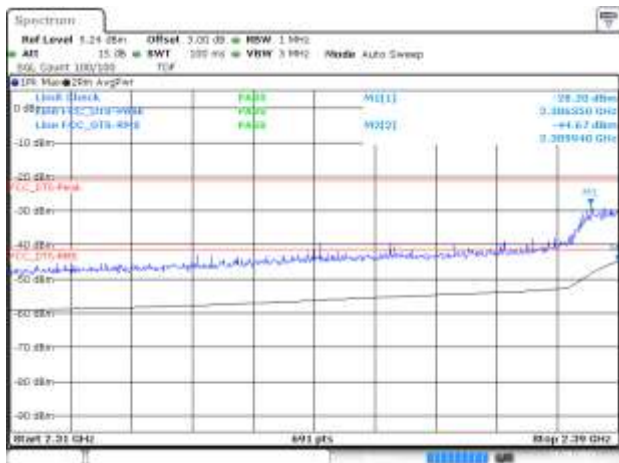
BE-R-LOW, MIMO-A, 802.11ax20-MCS0, Ch1
