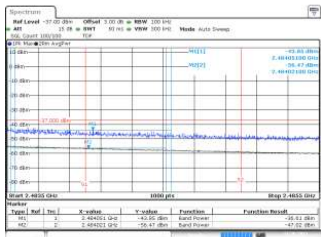
BE-R-HIGH-2MHz, MIMO-A, 802.11ax40-MCS0, Ch10
