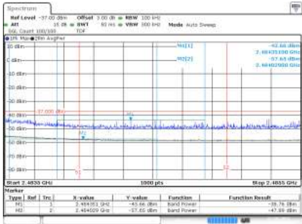
BE-R-HIGH-2MHz, MIMO-A, 802.11ax40-MCS0, Ch11
