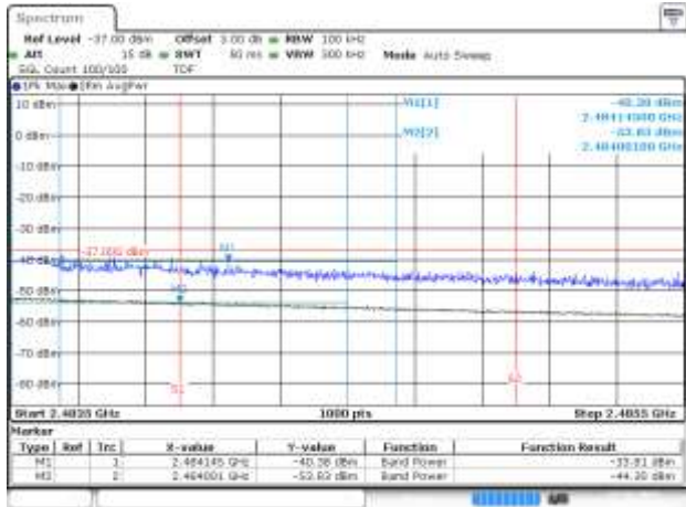
BE-R-HIGH-2MHz, SISO-B, 802.11ax40-MCS0, Ch10
