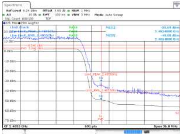
BE-R-HIGH, MIMO-B, 802.11ax20-MCS0, Ch13
