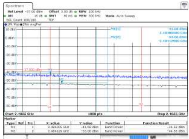
BE-R-HIGH-2MHz, MIMO-A, 802.11ax20-MCS0, Ch11
