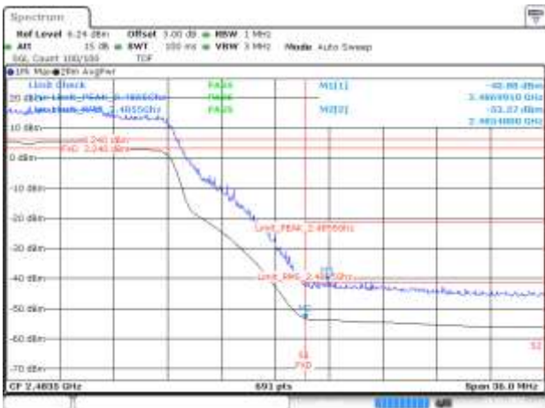
BE-R-HIGH, MIMO-B, 802.11ax20-MCS0, Ch12
