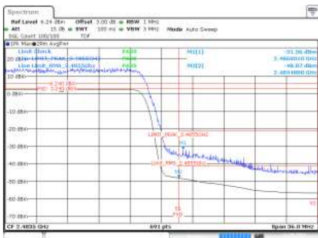
BE-R-HIGH, MIMO-A, 802.11ax20-MCS0, Ch13
