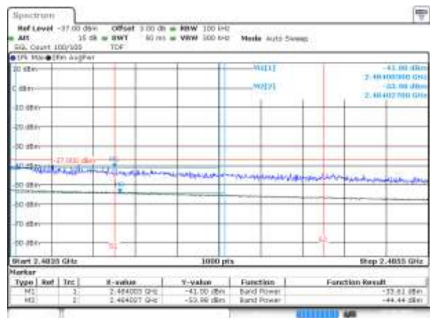
BE-R-HIGH-2MHz, SISO-A, 802.11ax40-MCS0, Ch10
