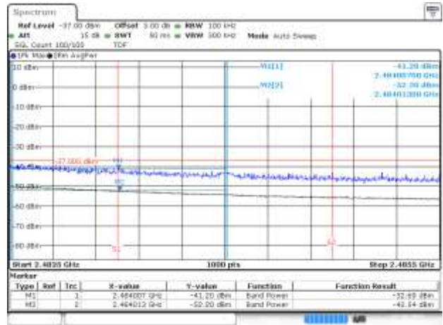
BE-R-HIGH-2MHz, SISO-A, 802.11ax20-MCS0, Ch12
