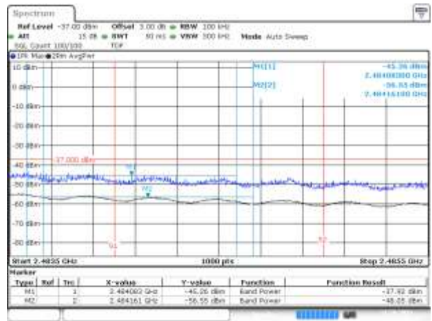
BE-R-HIGH-2MHz, MIMO-A, 802.11n40-HT8, Ch10
