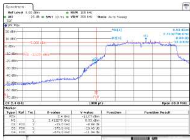
BE-NR, SISO-A, 802.11ax20-MCS0, Ch1
