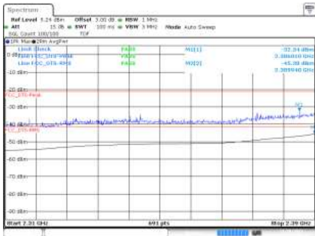
BE-R-LOW, MIMO-A, 802.11ax40-MCS0, Ch3
