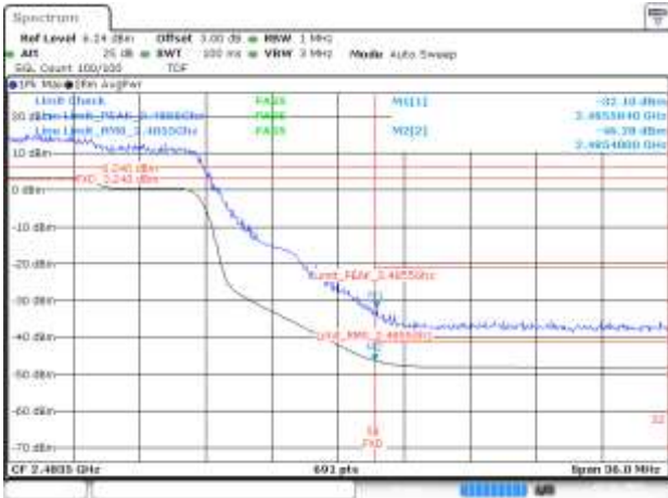
BE-R-HIGH, SISO-B, 802.11ax40-MCS0, Ch10
