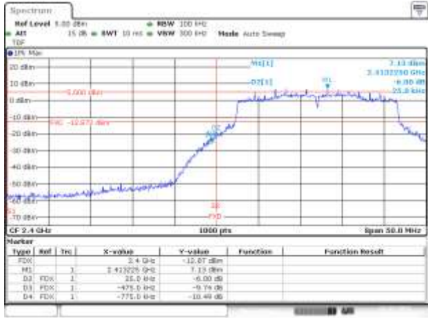
BE-NR, MIMO-B, 802.11ax20-MCS0, Ch1
