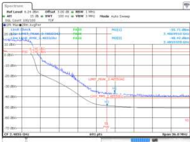
BE-R-HIGH, MIMO-A, 802.11ax40-MCS0, Ch9
