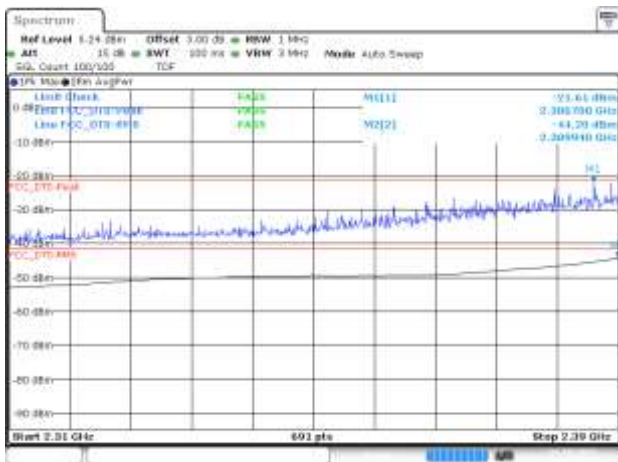
BE-R-LOW, SISO-A, 802.11ax40-MCS0, Ch3
