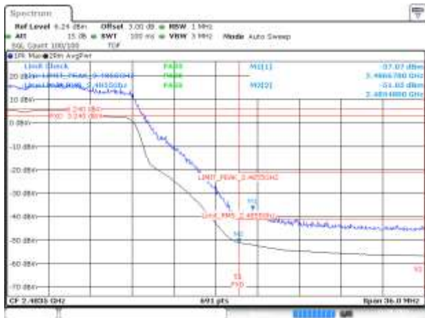
BE-R-HIGH, MIMO-A, 802.11ax20-MCS0, Ch12
