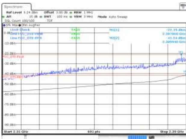
BE-R-LOW, SISO-B, 802.11ax20-MCS0, Ch1
