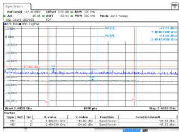
-BE-R-HIGH-2MHz, SISO-B, 802.11ax20-MCS0, Ch13
