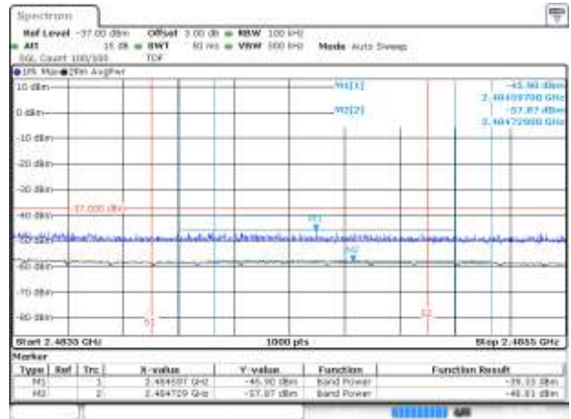
BE-R-HIGH-2MHz, MIMO-B, 802.11ax20-MCS0, Ch13
