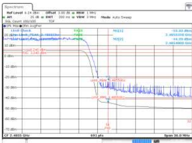
BE-R-HIGH, SISO-B, 802.11ax20-MCS0, Ch13
