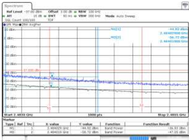
BE-R-HIGH-2MHz, MIMO-B, 802.11ax20-MCS0, Ch12
