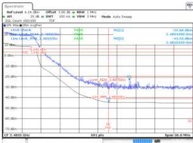
BE-R-HIGH, SISO-A, 802.11ax20-MCS0, Ch11
