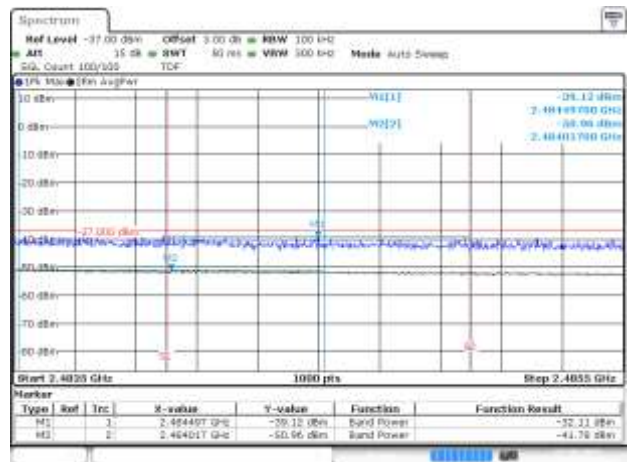
BE-R-HIGH-2MHz, SISO-B, 802.11ax20-MCS0, Ch11
