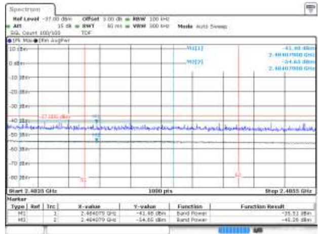
-BE-R-HIGH-2MHz, SISO-A, 802.11ax20-MCS0, Ch13
