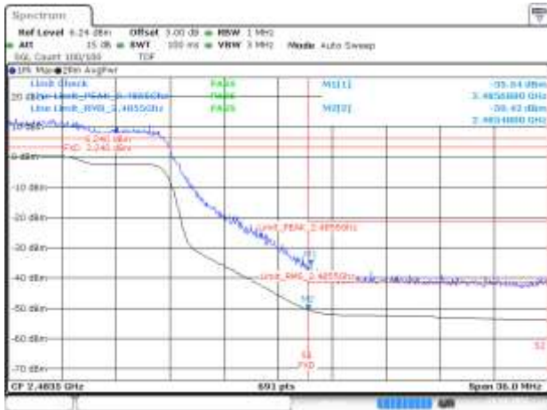
BE-R-HIGH, MIMO-B, 802.11ax40-MCS0, Ch10
