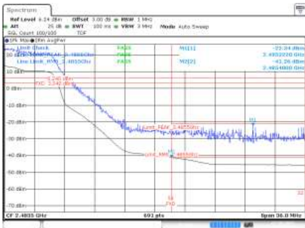
BE-R-HIGH, SISO-B, 802.11ax20-MCS0, Ch11
