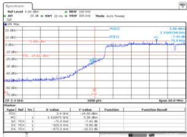
BE-NR, SISO-A, 802.11ax40-MCS0, Ch3
