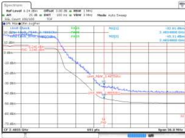
BE-R-HIGH, SISO-A, 802.11ax20-MCS0, Ch12
