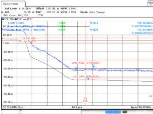
BE-R-HIGH, SISO-B, 802.11ax40-MCS0, Ch9
