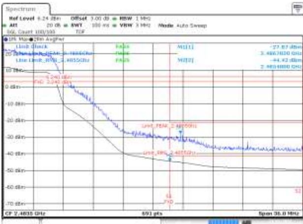
BE-R-HIGH, MIMO-B, 802.11ax20-MCS0, Ch11
