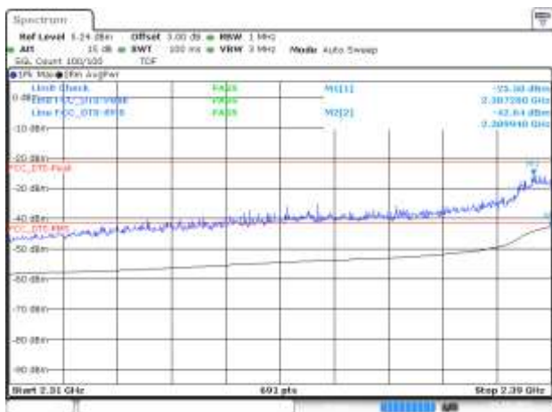
BE-R-LOW, SISO-A, 802.11ax20-MCS0, Ch1
