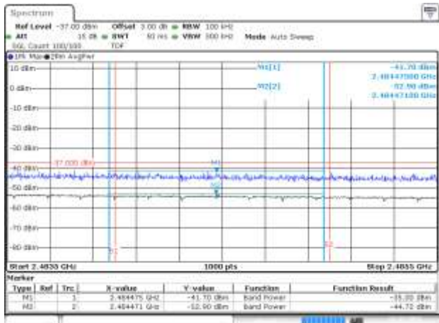
BE-R-HIGH-2MHz, MIMO-B, 802.11ax20-MCS0, Ch11
