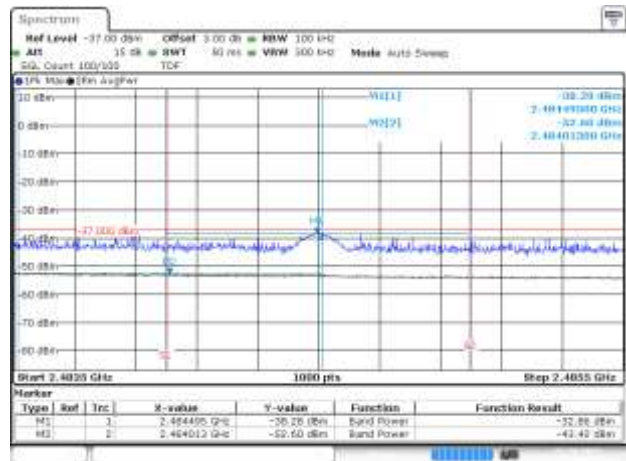
BE-R-HIGH-2MHz, SISO-A, 802.11ax40-MCS0, Ch9
