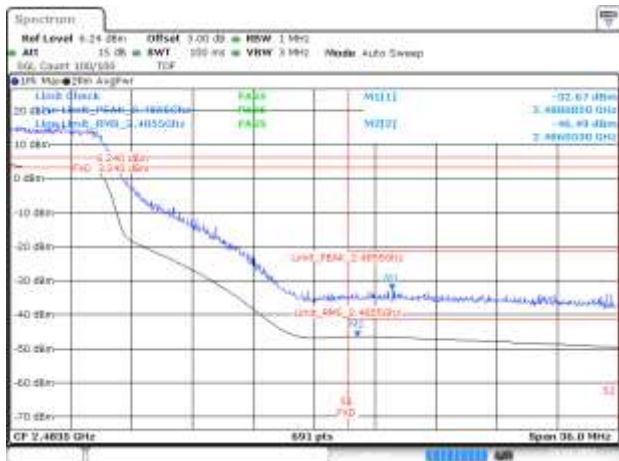
BE-R-HIGH, MIMO-B, 802.11ax40-MCS0, Ch9
