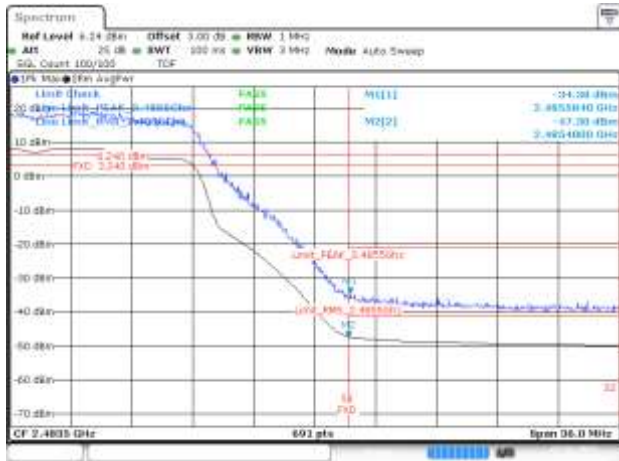
BE-R-HIGH, SISO-B, 802.11ax20-MCS0, Ch12
