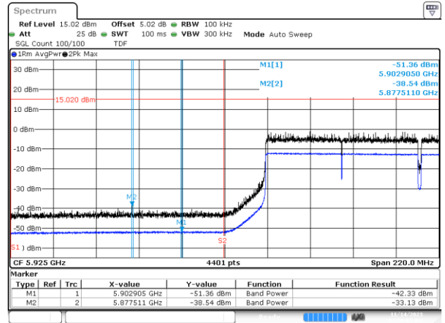
BE-NR-LOW, SISO-B, 802.11ax160-HE0, Ch15
