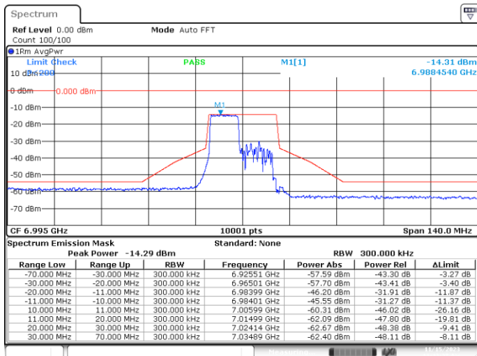
MIMO-B, 802.11ax/be20-MCS0, Ch209-8m-53
