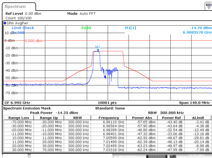
MIMO-B, 802.11ax/be20-MCS0, Ch209-4m-37
