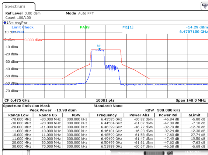
MIMO-A, 802.11ax/be20-MCS0, Ch105-8m-53
