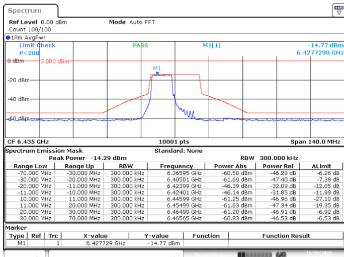
MIMO-A, 802.11ax/be20-MCS0, Ch97-8m-53
