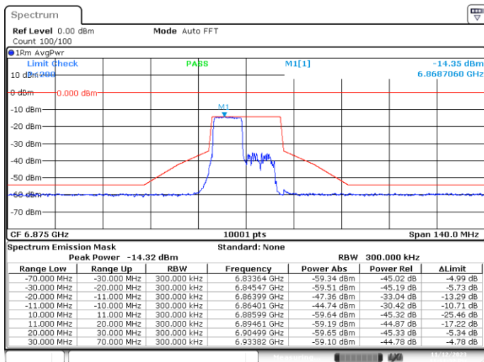
MIMO-A, 802.11ax/be20-MCS0, Ch185-8m-53
