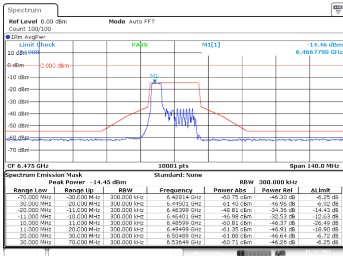
MIMO-A, 802.11ax/be20-MCS0, Ch105-4m-37
