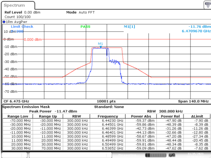
SISO-B, 802.11ax/be20-MCS0, Ch105-10m-2
