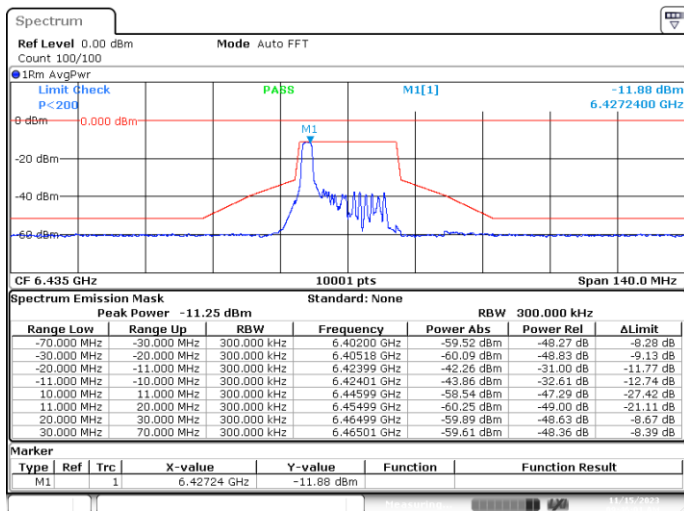
SISO-B, 802.11ax/be20-MCS0, Ch97-2m-0
