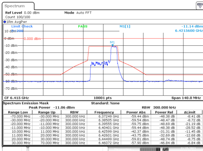
SISO-B, 802.11ax/be20-MCS0, Ch93-4m-37
