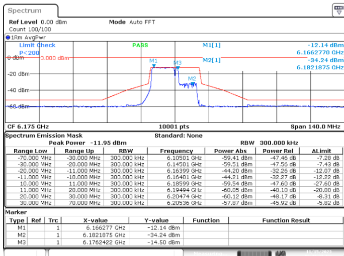
SISO-B, 802.11ax/be20-MCS0, Ch45-10m-82
