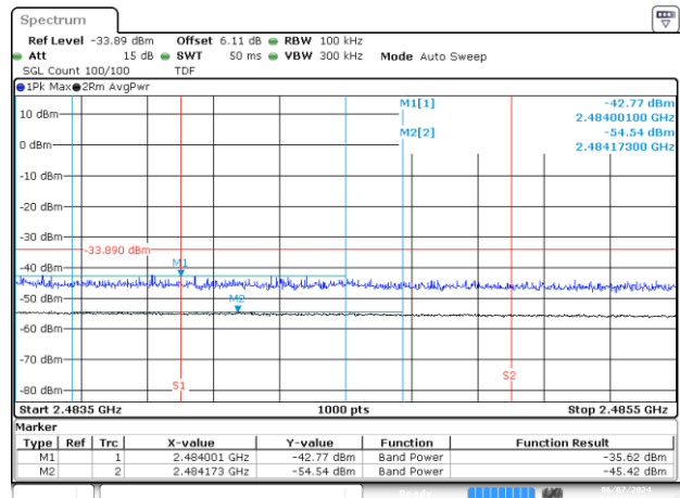
BE-R-HIGH-2MHz, MIMO-B, 802.11ax/be20-MCS0, Ch11
