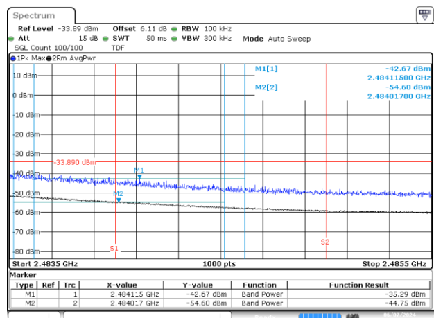
BE-R-HIGH-2MHz, MIMO-B, 802.11ax/be20-MCS0, Ch12
