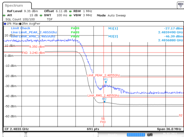
Date 7.JUN.2014 16:33:03 BE-R-HIGH, MIMO-B, 802.11ax/be40-MCS0, Ch11
