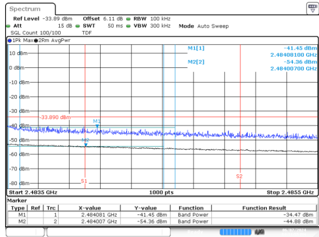
Date 7.JUN.2014 16:31:55 BE-R-HIGH-2MHz, MIMO-B, 802.11ax/be40-MCS0, Ch10
