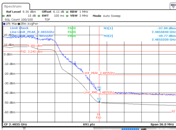
BE-R-HIGH, MIMO-B, 802.11ax/be20-MCS0, Ch12
