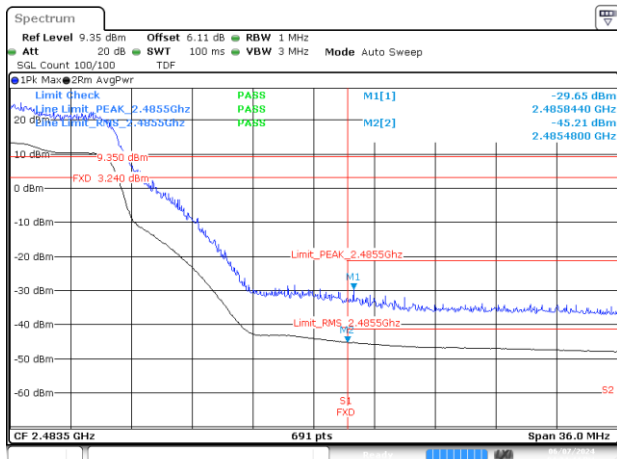
BE-R-HIGH, MIMO-B, 802.11ax/be20-MCS0, Ch11
