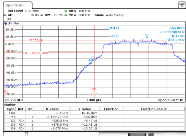
BE-NR, MIMO-B, 802.11ax/be20-MCS0, Ch1
