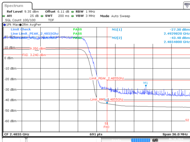
BE-R-HIGH, SISO-B, 802.11ax/be20-MCS0, Ch13
