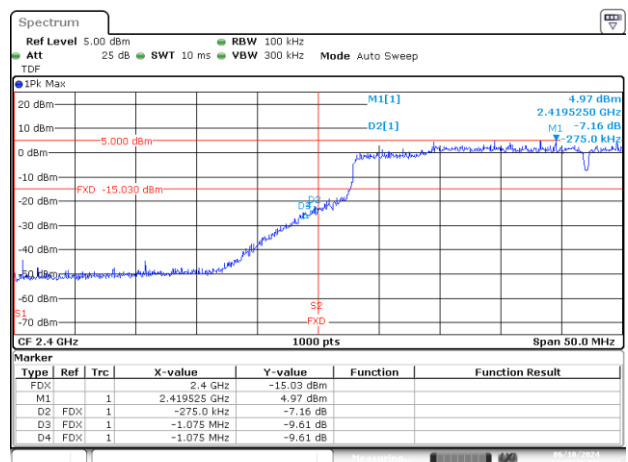
BE-NR, SISO-B, 802.11ax/be40-MCS0, Ch3
