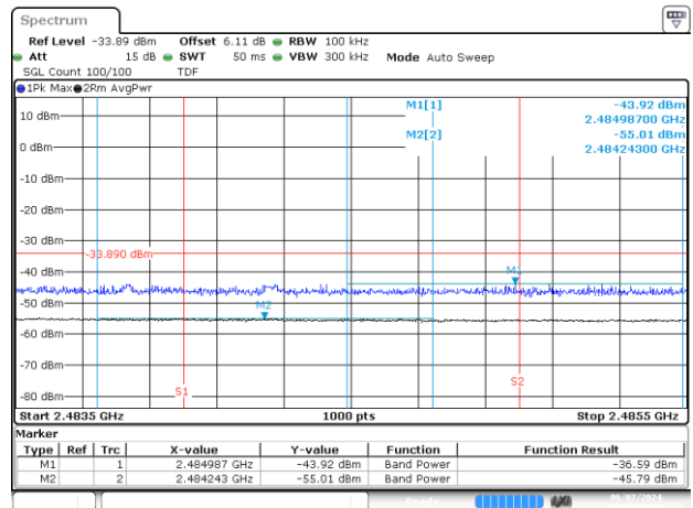
BE-R-HIGH-2MHz, MIMO-A, 802.11ax/be40-MCS0, Ch9
