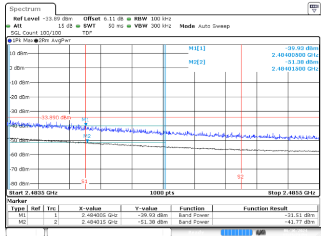
BE-R-HIGH-2MHz, SISO-B, 802.11ax/be20-MCS0, Ch12
