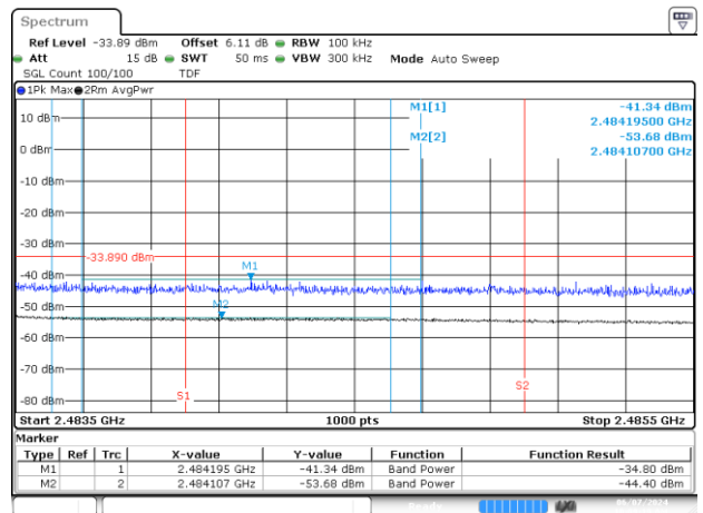
Date 7.JUN.2024 10:03:19 BE-R-HIGH-2MHz, MIMO-A, 802.11ax/be20-MCS0, Ch13
