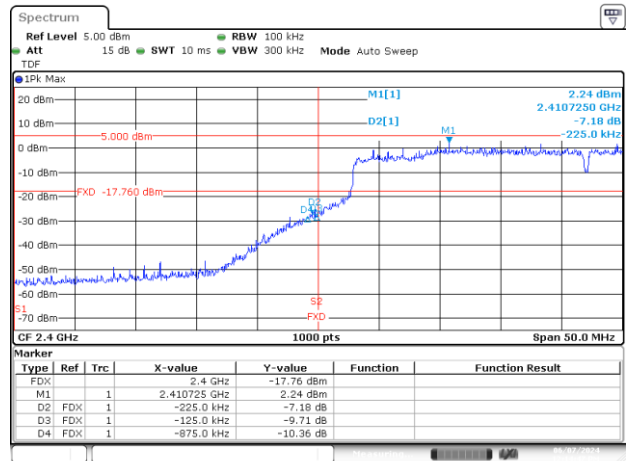
BE-NR, MIMO-A, 802.11ax/be40-MCS0, Ch3
