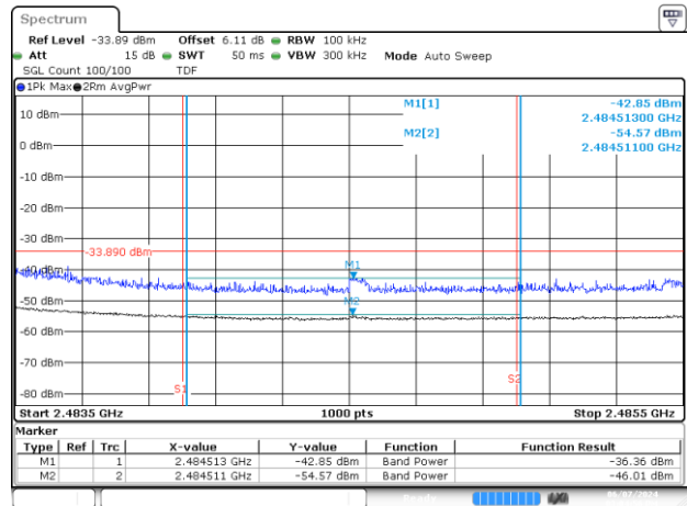
BE-R-HIGH-2MHz, MIMO-A, 802.11ax/be40-MCS0, Ch11
