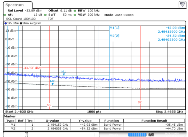
Date 7.JUN.2024 11:52:14 BE-R-HIGH-2MHz, MIMO-A, 802.11ax/be20-MCS0, Ch12
