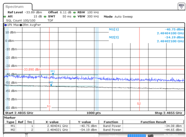
BE-R-HIGH-2MHz, MIMO-A, 802.11ax/be40-MCS0, Ch10
