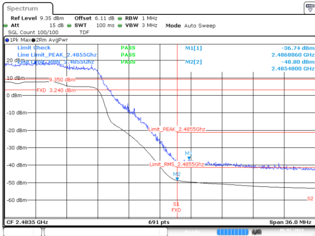
Date 7.JUN.2024 11:52:07 BE-R-HIGH, MIMO-A, 802.11ax/be20-MCS0, Ch12
