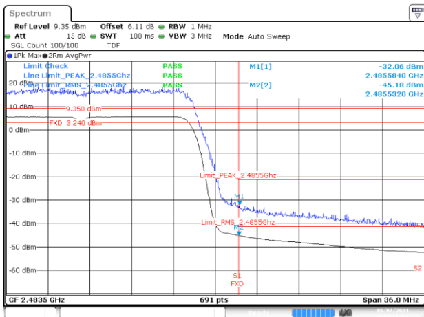
Date 7.JUN.2024 10:03:13 BE-R-HIGH, MIMO-A, 802.11ax/be20-MCS0, Ch13
