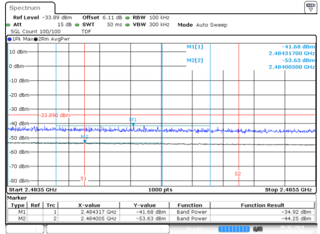
Date 7.JUN.2024 12:03:51 BE-R-HIGH-2MHz, MIMO-A, 802.11ax/be20-MCS0, Ch11
