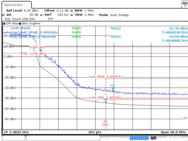
Date 7.JUN.2024 12:03:45 BE-R-HIGH, MIMO-A, 802.11ax/be20-MCS0, Ch11
