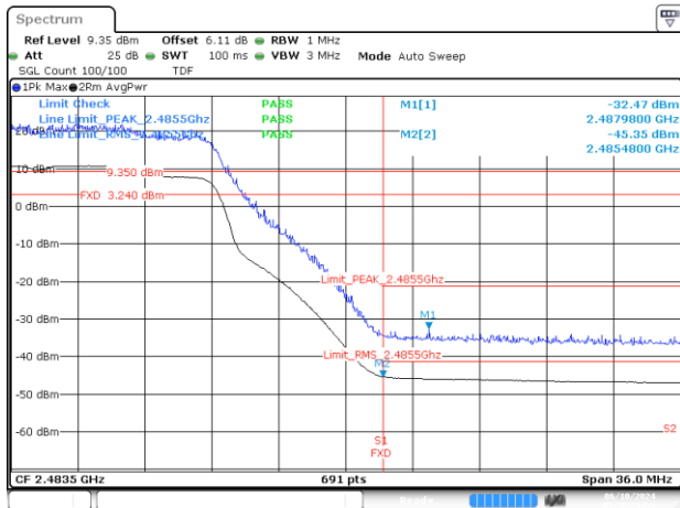
BE-R-HIGH, SISO-B, 802.11ax/be20-MCS0, Ch12
