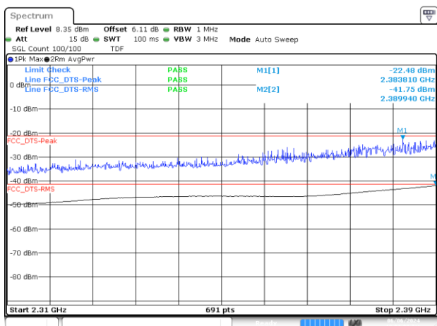
Date 6.JUN.2024 10:03:04 BE-R-LOW, SISO-A, 802.11ax/be40-MCS0, Ch3
