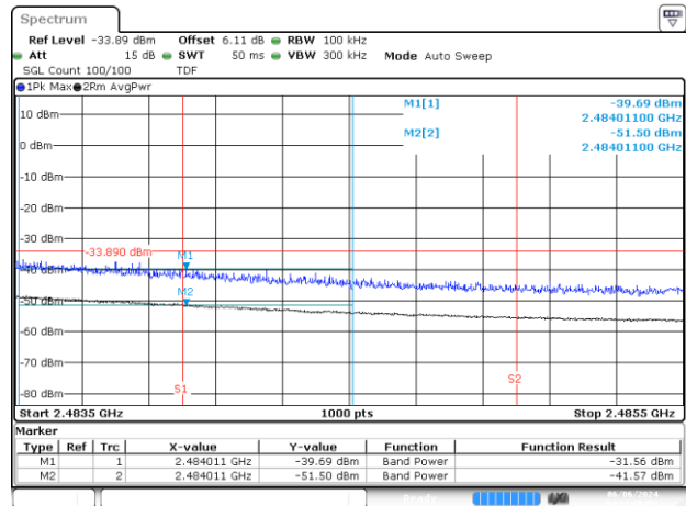
Date 6.JUN.2024 16:23:05 BE-R-HIGH-2MHz, SISO-A, 802.11ax/be20-MCS0, Ch12
