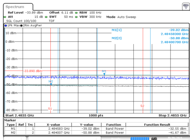
BE-R-HIGH-2MHz, SISO-A, 802.11ax/be20-MCS0, Ch11
