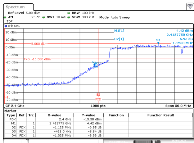
Date 6.JUN.2024 10:03:11 BE-NR, SISO-A, 802.11ax/be40-MCS0, Ch3
