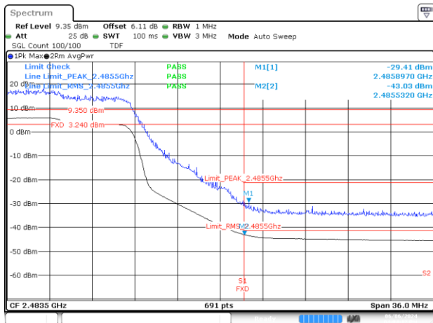
Date 6.JUN.2024 13:04:12 BE-R-HIGH, SISO-A, 802.11ax/be40-MCS0, Ch10
