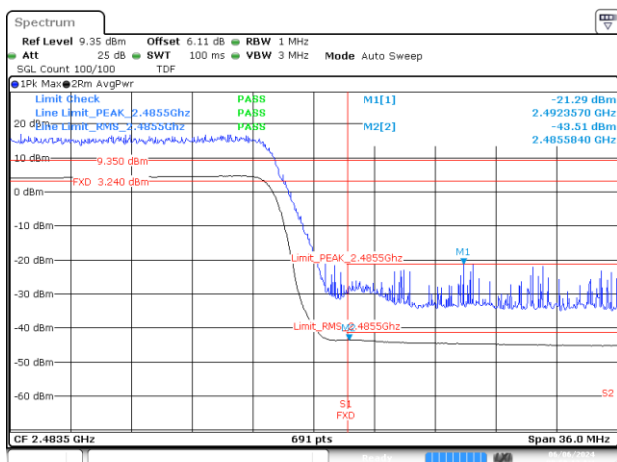
Date 6.JUN.2024 09:58:13 BE-R-HIGH, SISO-A, 802.11ax/be40-MCS0, Ch11
