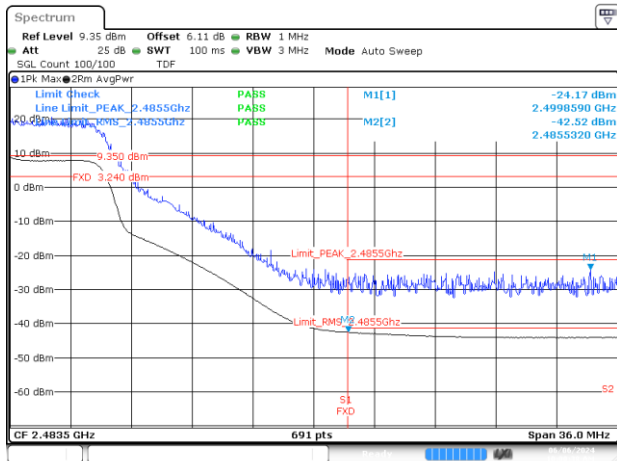
Date 6.JUN.2024 10:03:39 BE-R-HIGH, SISO-A, 802.11ax/be40-MCS0, Ch9
