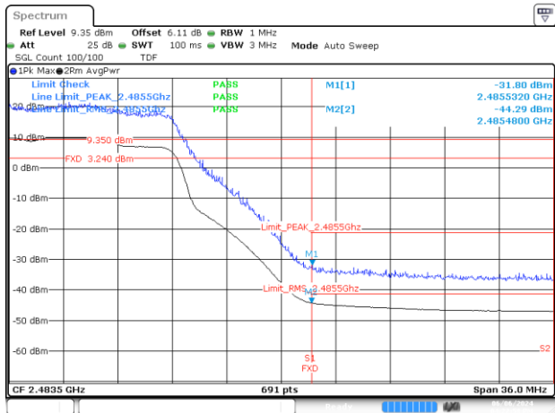
Date 6.JUN.2024 16:23:58 BE-R-HIGH, SISO-A, 802.11ax/be20-MCS0, Ch12
