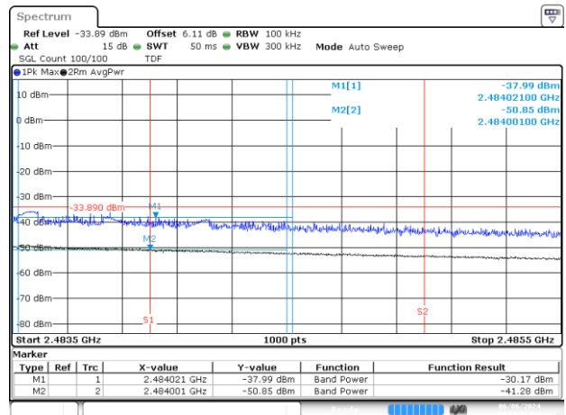
Date 6.JUN.2024 13:04:19 BE-R-HIGH-2MHz, SISO-A, 802.11ax/be40-MCS0, Ch10
