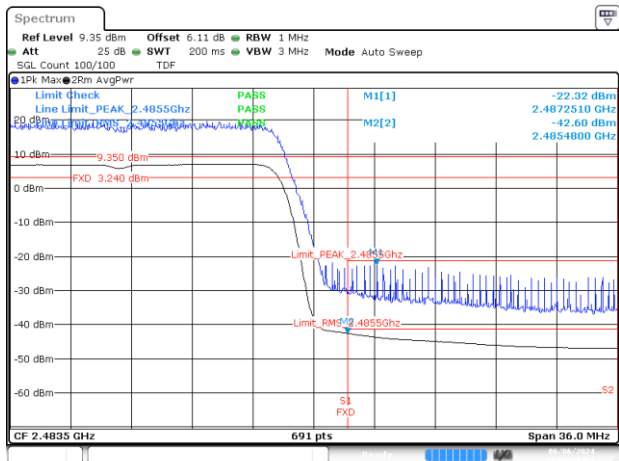
Date 6.JUN.2024 10:04:25 BE-R-HIGH, SISO-A, 802.11ax/be20-MCS0, Ch13
