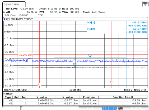
Date 6.JUN.2024 10:00:46 BE-R-HIGH-2MHz, SISO-A, 802.11ax/be40-MCS0, Ch9
