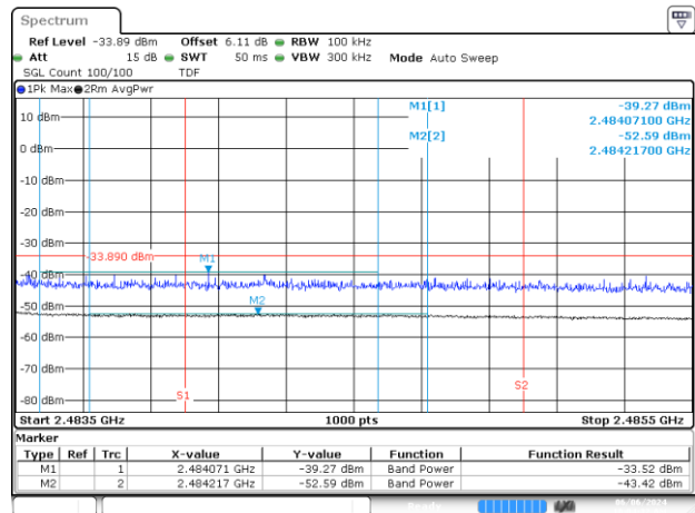
Date 6.JUN.2024 10:04:31 -BE-R-HIGH-2MHz, SISO-A, 802.11ax/be20-MCS0, Ch13
