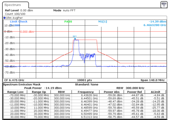
MIMO-A, 802.11ax/be20-MCS0, Ch105-4m-37
