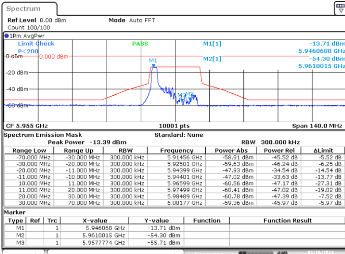
MIMO-A, 802.11ax/be20-MCS0, Ch1-2m-0
