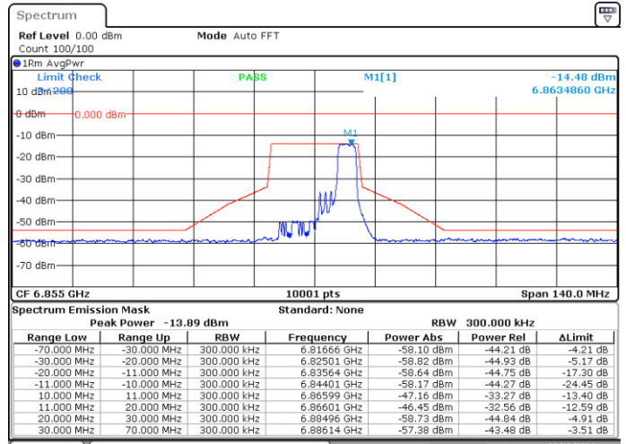
MIMO-A, 802.11ax/be20-MCS0, Ch181-4m-37
