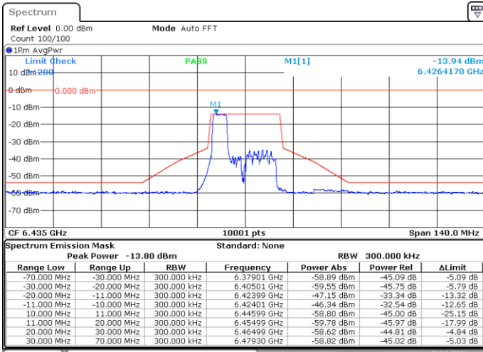
MIMO-A, 802.11ax/be20-MCS0, Ch97-4m-37
