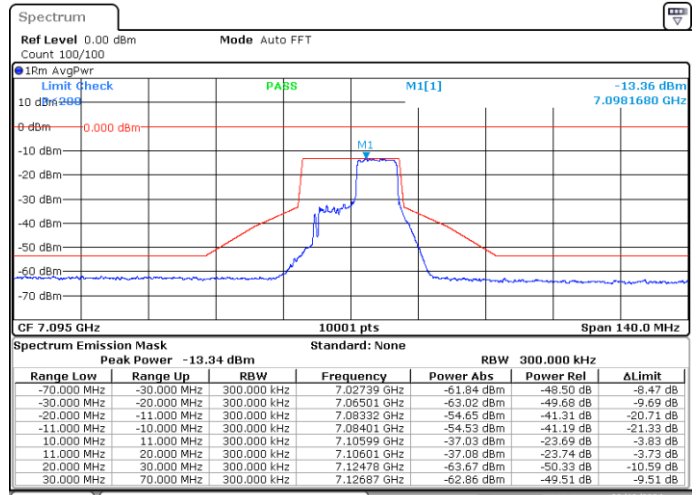
MIMO-A, 802.11ax/be20-MCS0, Ch229-8m-54
