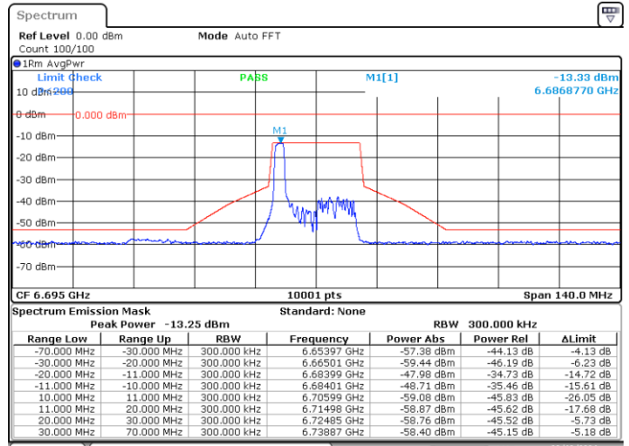
MIMO-A, 802.11ax/be20-MCS0, Ch149-2m-0
