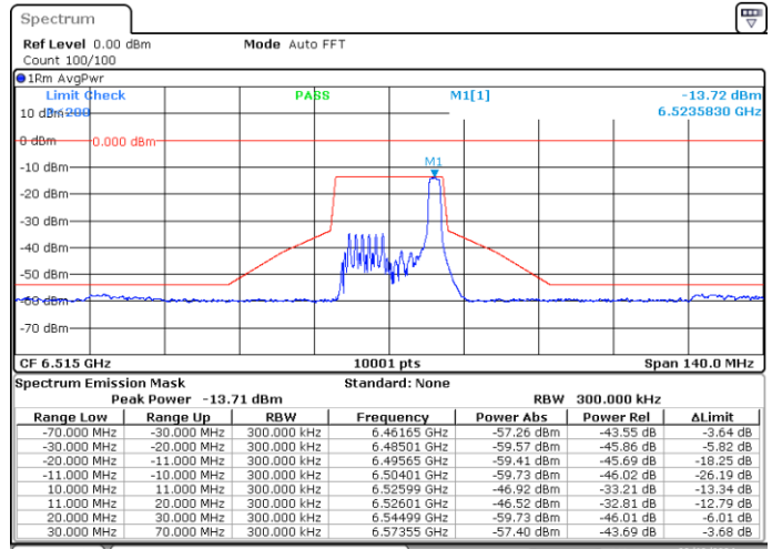
MIMO-A, 802.11ax/be20-MCS0, Ch113-2m-0
