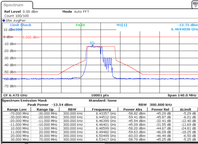
MIMO-A, 802.11ax/be20-MCS0, Ch105-10m-82
