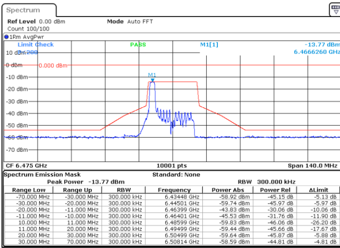
MIMO-A, 802.11ax/be20-MCS0, Ch105-2m-0
