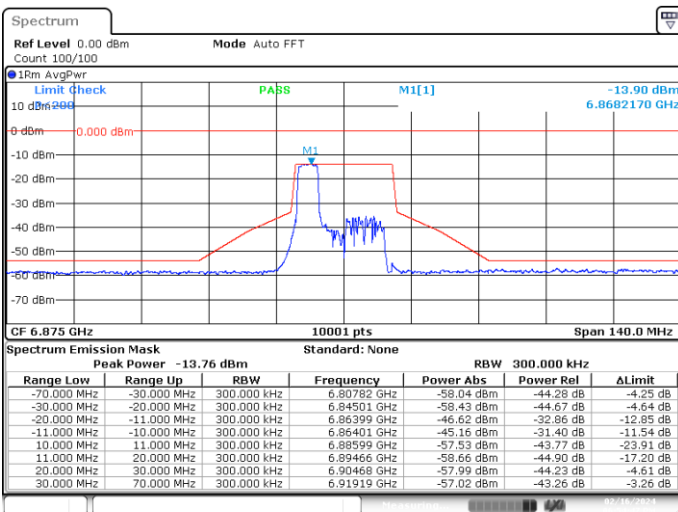
MIMO-A, 802.11ax/be20-MCS0, Ch185-4m-37
