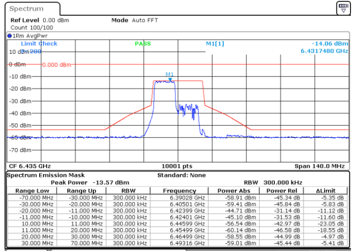
MIMO-A, 802.11ax/be20-MCS0, Ch97-8m-53
