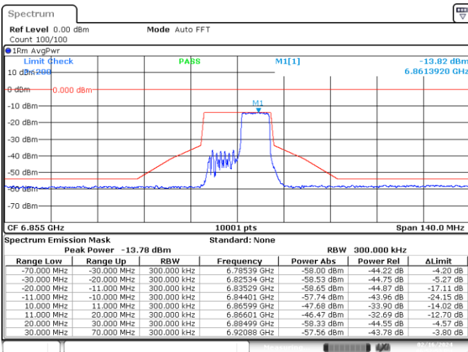
MIMO-A, 802.11ax/be20-MCS0, Ch181-8m-53
