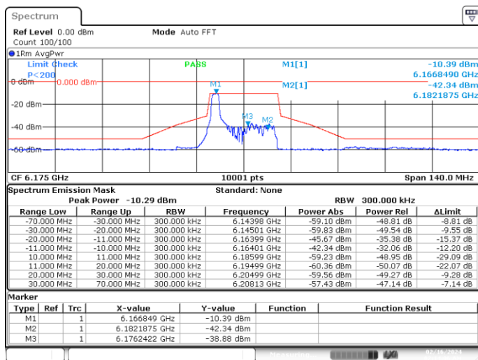
SISO-B, 802.11ax/be20-MCS0, Ch45-2m-0
