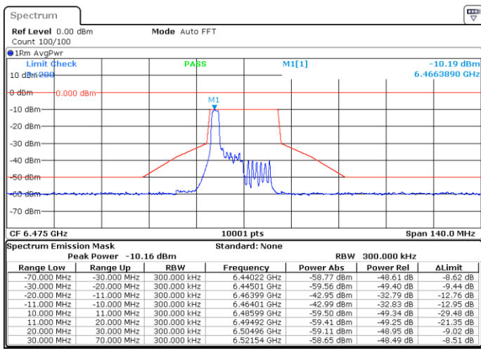
SISO-B, 802.11ax/be20-MCS0, Ch105-2m-0
