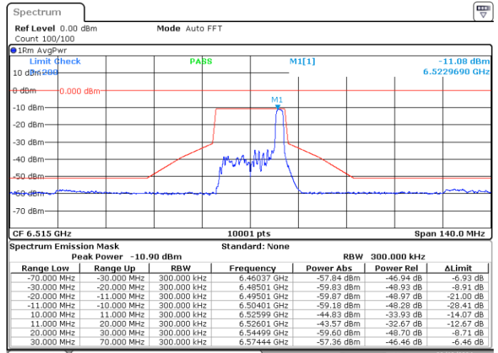
SISO-B, 802.11ax/be20-MCS0, Ch113-2m-0
