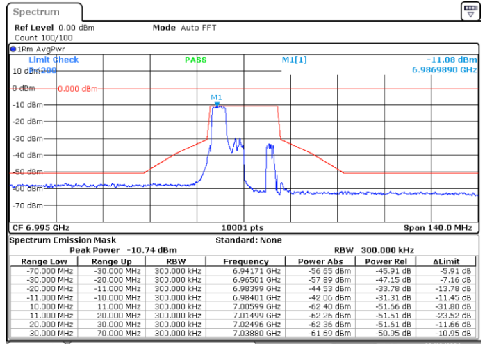
SISO-A, 802.11ax/be20-MCS0, Ch209-4m-37
