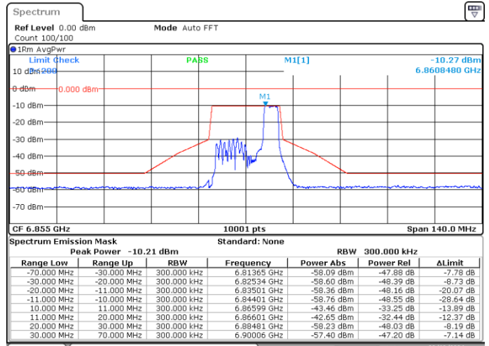
SISO-A, 802.11ax/be20-MCS0, Ch181-4m-37
