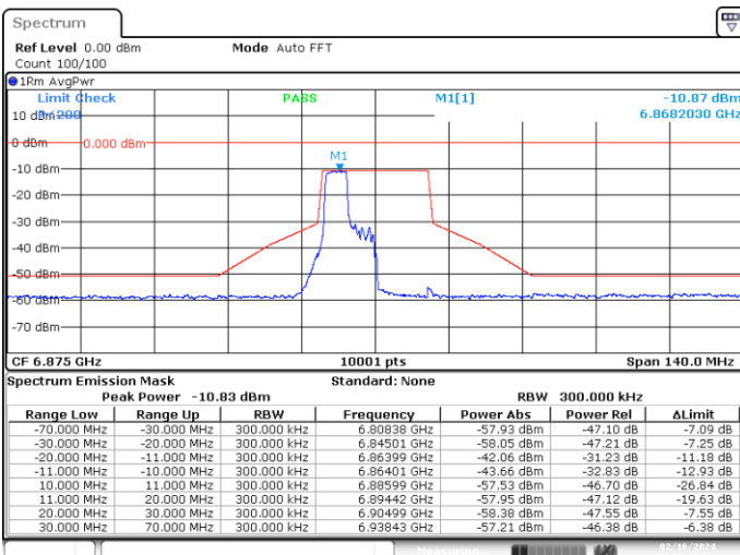
SISO-A, 802.11ax/be20-MCS0, Ch185-4m-37
