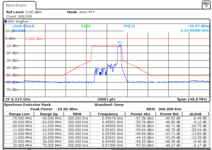
SISO-A, 802.11ax/be20-MCS0, Ch113-2m-0
