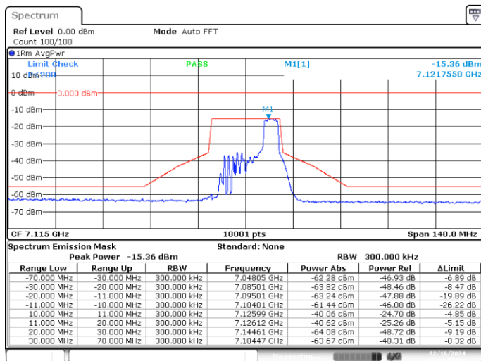
SISO-A, 802.11ax/be20-MCS0, Ch233-4m-40
