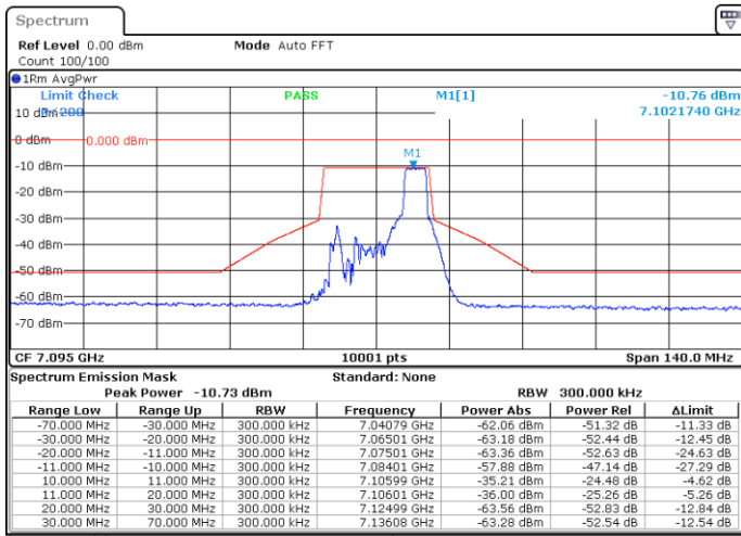
SISO-A, 802.11ax/be20-MCS0, Ch229-4m-40
