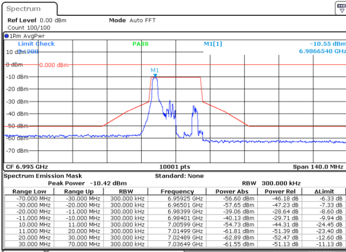
SISO-B, 802.11ax/be20-MCS0, Ch209-2m-0
