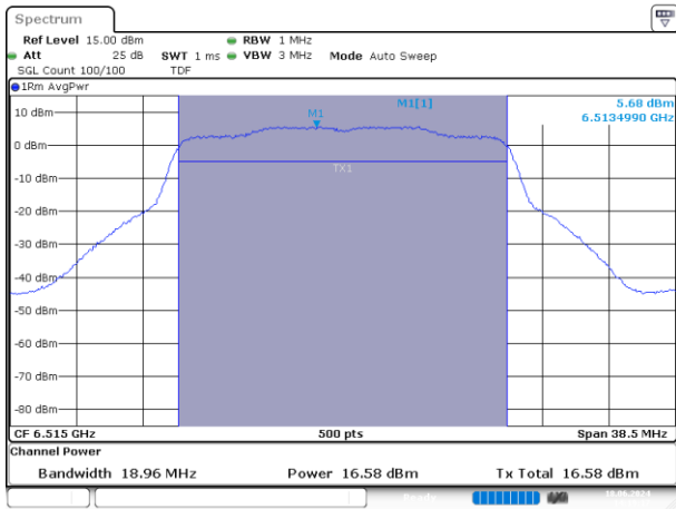
MIMO A-802.11ax/be-20MHz-Ch113-MCS0
