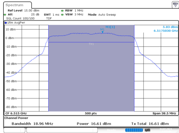
MIMO B-802.11ax/be-20MHz-Ch113-MCS0
