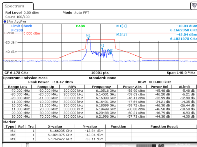
MIMO-A, 802.11ax/be20-MCS0, Ch45-2m-0
