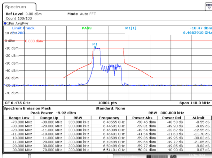
MIMO-B, 802.11ax/be20-MCS0, Ch105-4m-37
