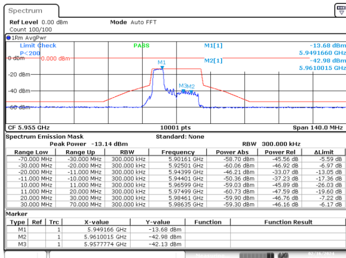
MIMO-A, 802.11ax/be20-MCS0, Ch1-4m-37
