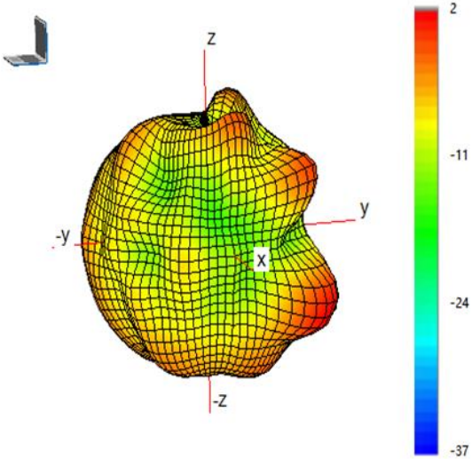
Max Antenna 3D Radiation Pattern 5150-5250 MHz
