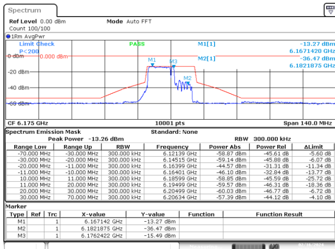
MIMO-A, 802.11ax/be20-MCS0, Ch45-10m-82
