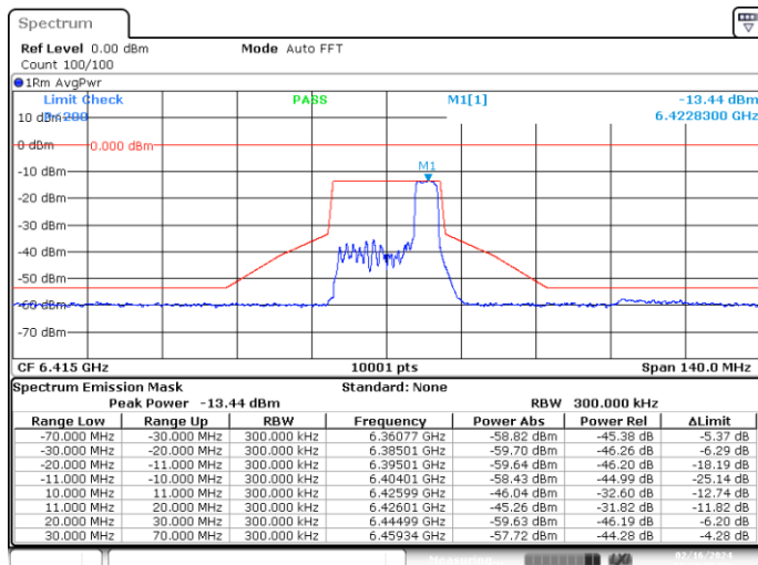
MIMO-A, 802.11ax/be20-MCS0, Ch93-4m-37
