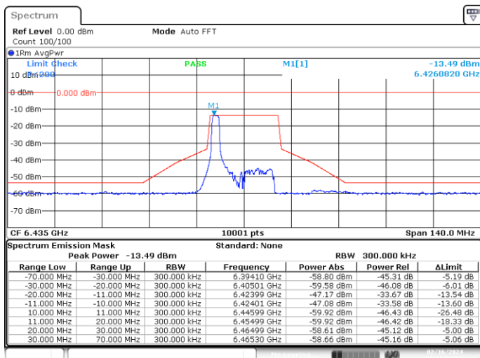
MIMO-A, 802.11ax/be20-MCS0, Ch97-2m-0
