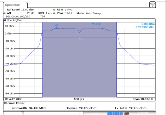
MIMO B-802.11n-40MHz-Ch46-5230MHz-HT8
