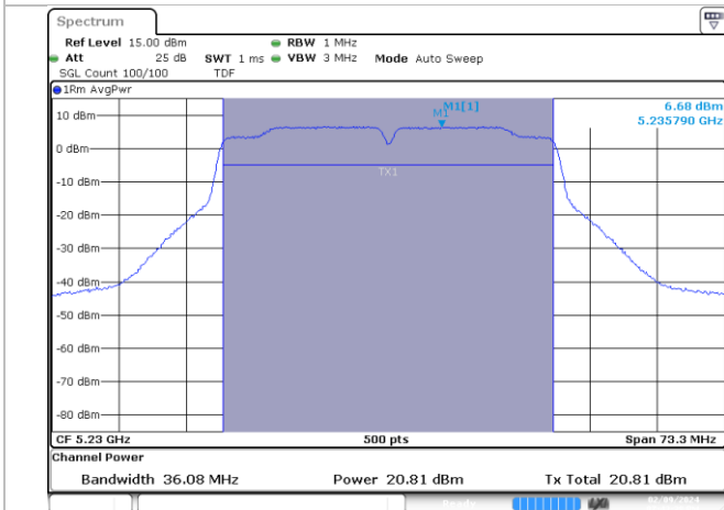
MIMO A-802.11n-40MHz-Ch46-5230MHz-HT8
