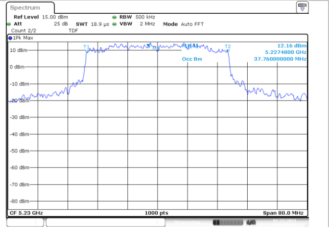
SISO A-802.11ax/be-40MHz-46-5230-MCS0 99%
