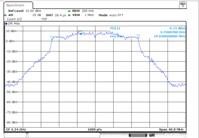
MIMO B-802.11ax/be-20MHz-48-5240-MCS0 99%
