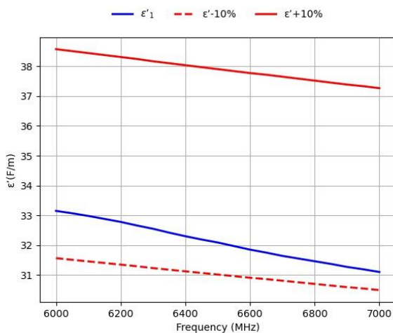
Permittivity 2024-01-22
