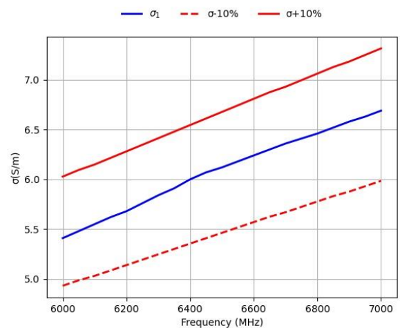
Conductivity 2024-01-22
