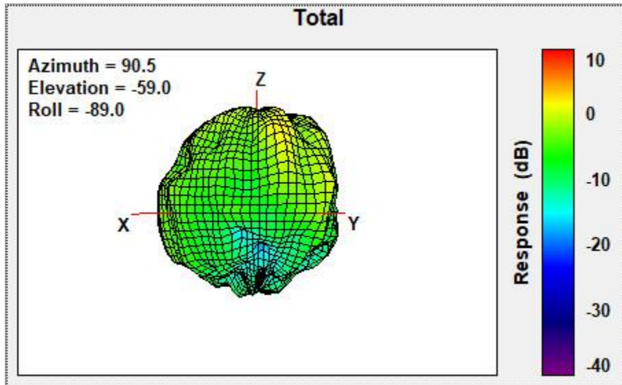
Max Antenna 3D Radiation Pattern 5250-5350 MHz
