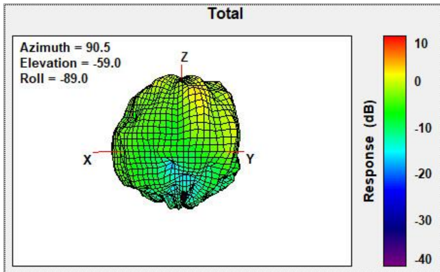
Max Antenna 3D Radiation Pattern 5470-5725 MHz
