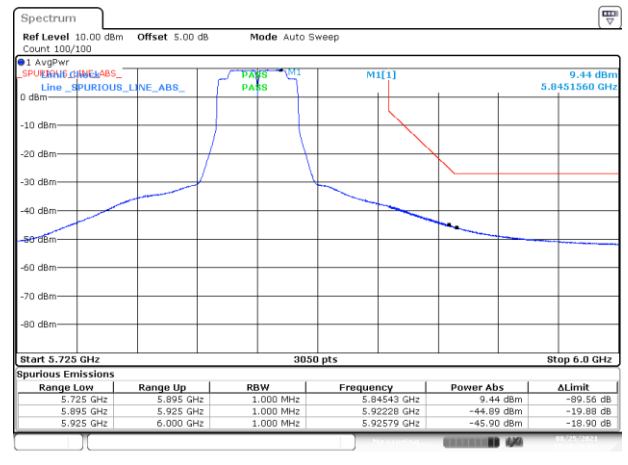
BE-NR-HIGH, MIMO-B, 802.11n40-HT0, Ch167
