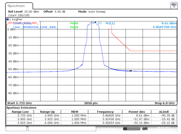
BE-NR-HIGH, MIMO-B, 802.11ax20-MCS0, Ch173
