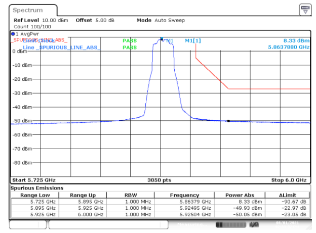
BE-NR-HIGH, MIMO-A, 802.11ax20-MCS0, Ch173
