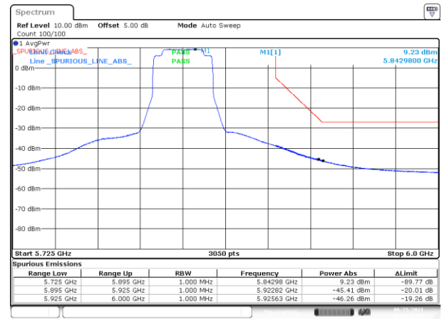
BE-NR-HIGH, MIMO-A, 802.11ax40-MCS0, Ch167
