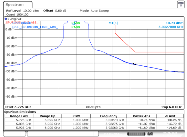
BE-NR-HIGH, SISO-A, 802.11ax40-MCS0, Ch167
