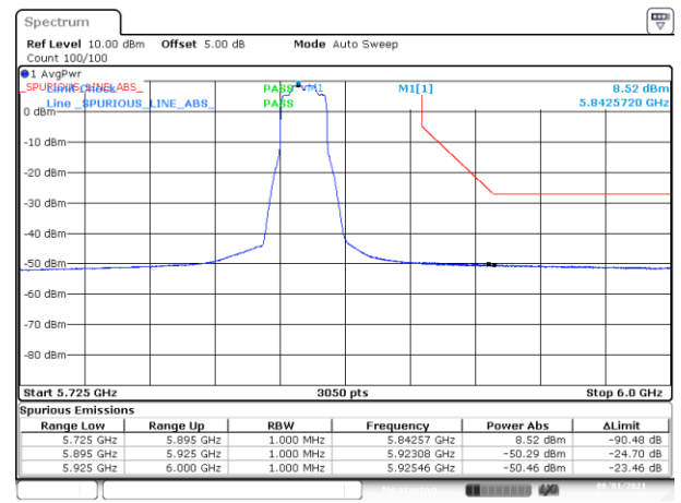
BE-NR-HIGH, MIMO-A, 802.11ax20-MCS0, Ch169
