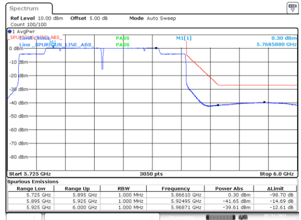
BE-NR-HIGH, SISO-A, 802.11ax160-MCS0, Ch163
