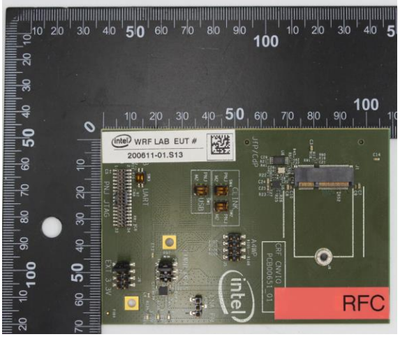
Extender board
