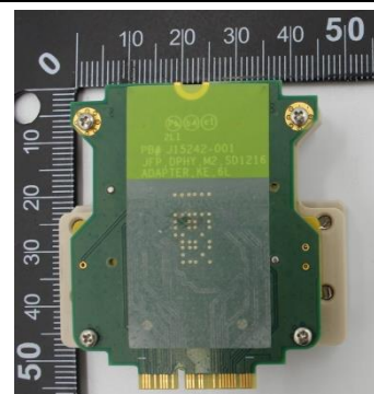
Socket Back
