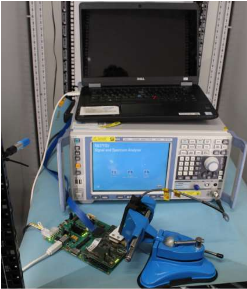
Conducted Setup
