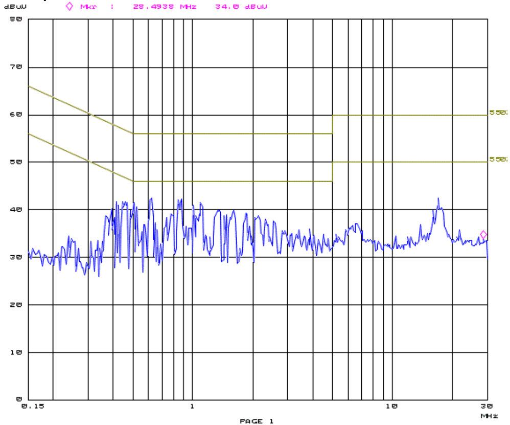
Plot 19: Pre-scan plot with peak detector. Conducted emissions from 0.15 - 30 MHz, 5GHz + BT mode
