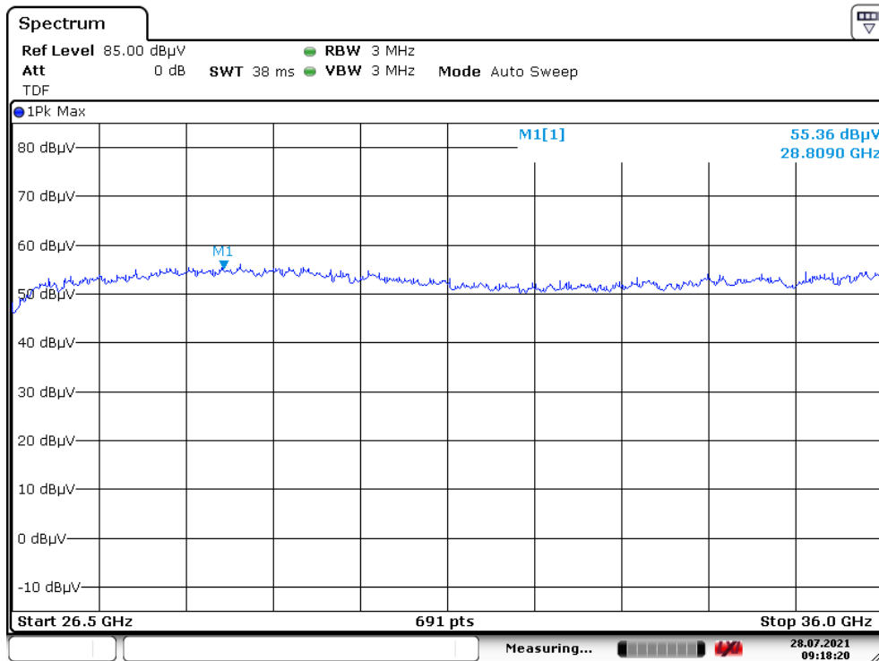
Plot 17: Pre-scan plot with peak detector Radiated emissions from 26.5 GHz – 36 GHz, 2.4GHz mode
