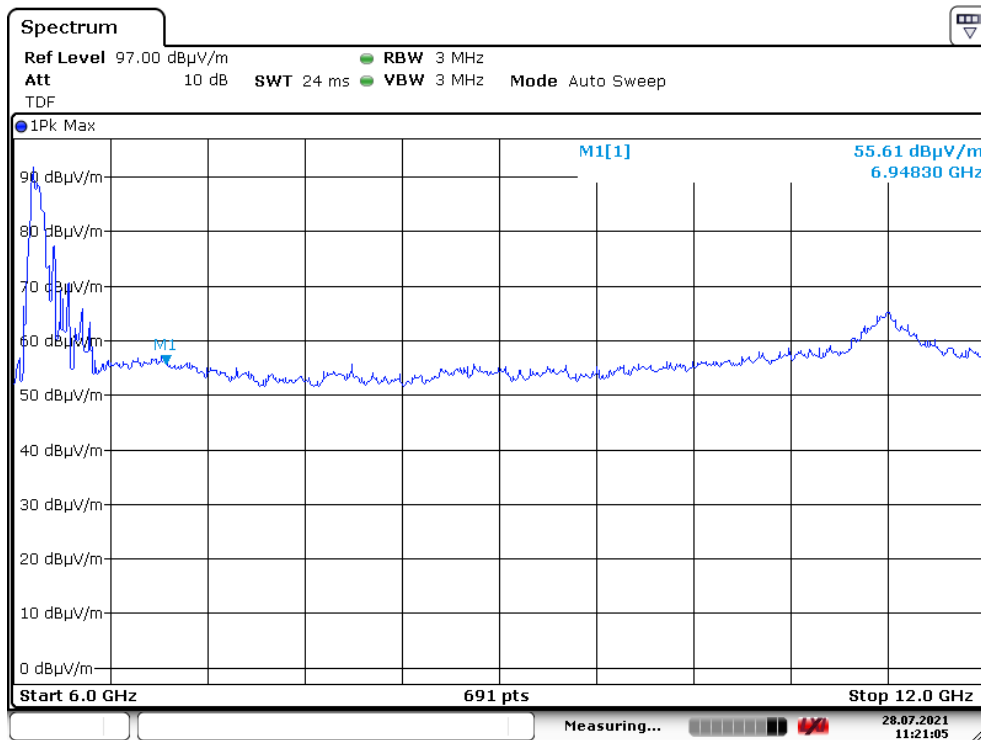
Plot 9: Pre-scan plot with peak detector. Radiated emissions from 6 GHz – 12 GHz, 6GHz mode
