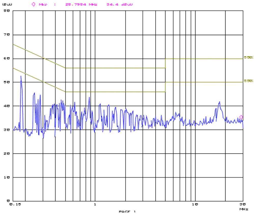
Plot 21: Pre-scan plot with peak detector. Conducted emissions from 0.15 - 30 MHz, 6GHz mode
