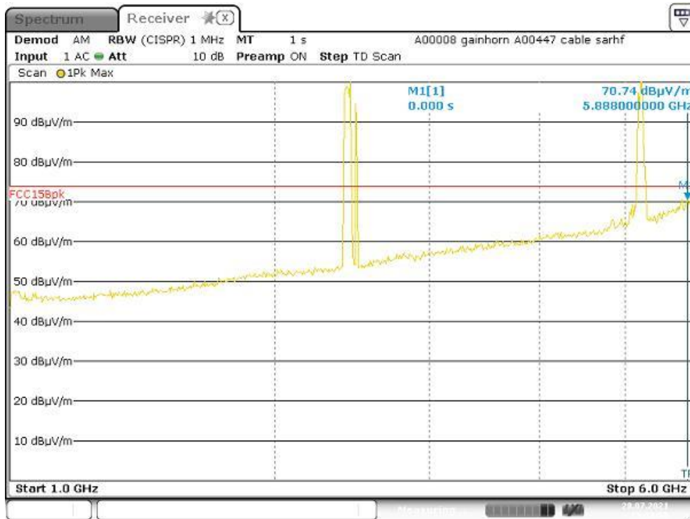
Plot 4: Pre-scan plot with peak detector. Radiated emissions from 1 GHz – 6 GHz, 5GHz + BT mode
