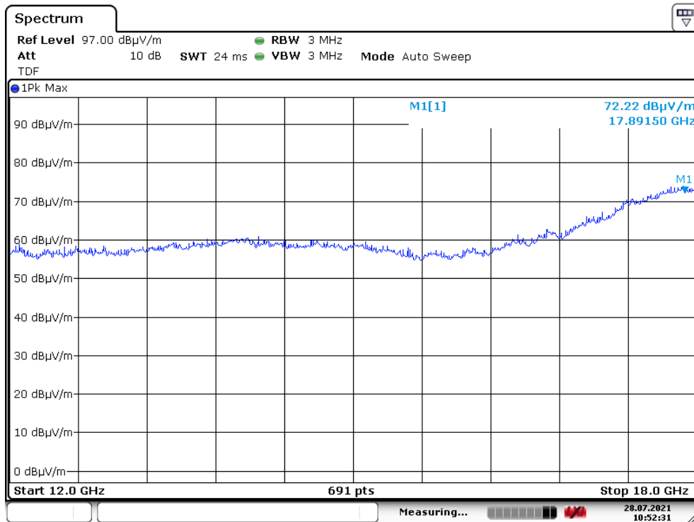
Plot 11: Pre-scan plot with peak detector. Radiated emissions from 12 GHz – 18 GHz, 2.4GHz mode
