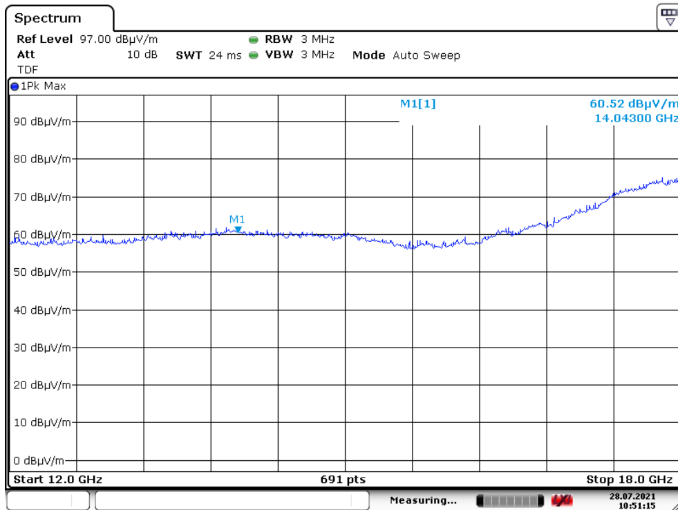
Plot 10: Pre-scan plot with peak detector. Radiated emissions from 12 GHz – 18 GHz, 5GHz + BT mode
