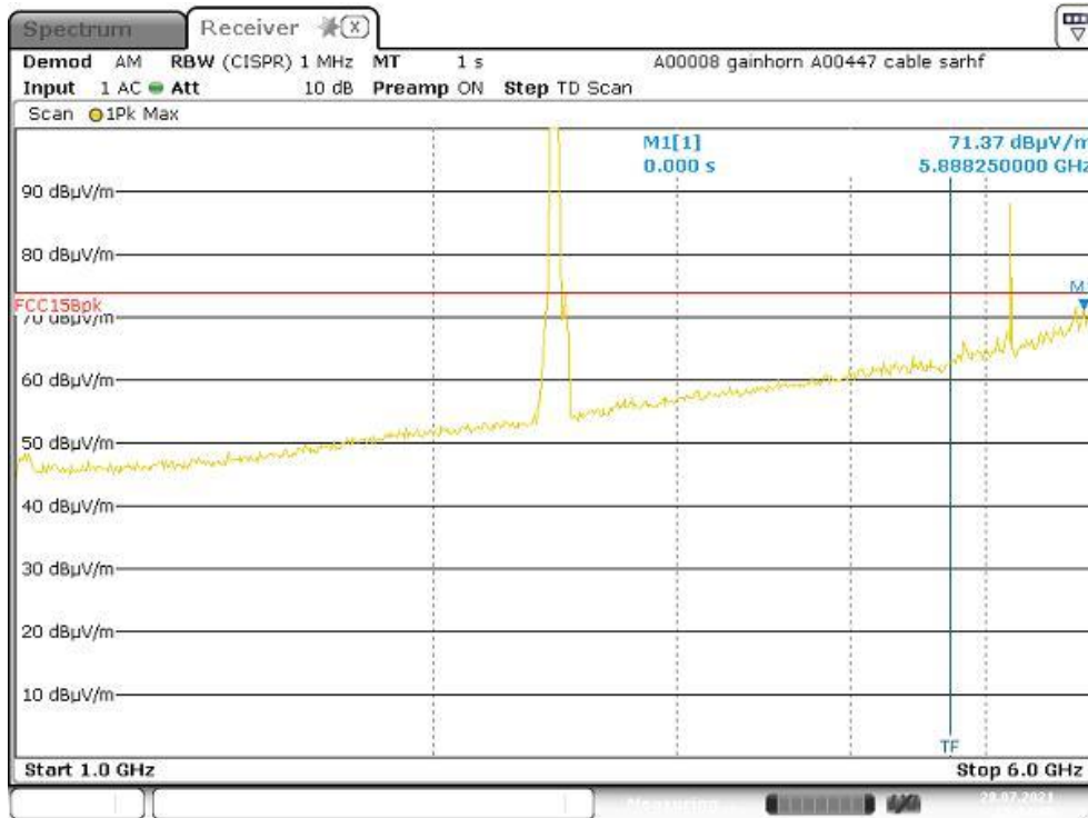
Plot 5: Pre-scan plot with peak detector. Radiated emissions from 1 GHz – 6 GHz, 2.4GHz mode
