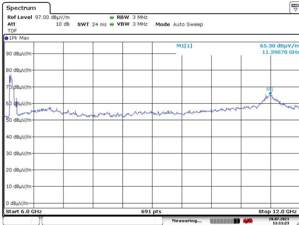
Plot 8: Pre-scan plot with peak detector. Radiated emissions from 6 GHz – 12 GHz, 2.4GHz mode
