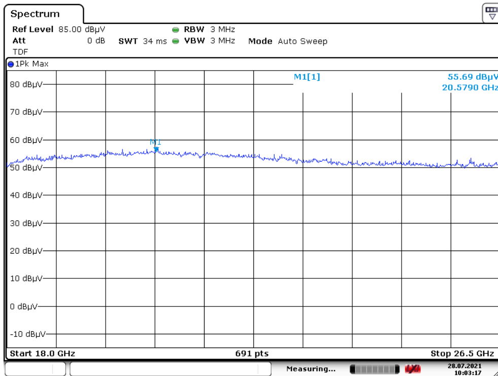
Plot 14: Pre-scan plot with peak detector. Radiated emissions from 18 GHz – 26.5 GHz, 2.4GHz mode
