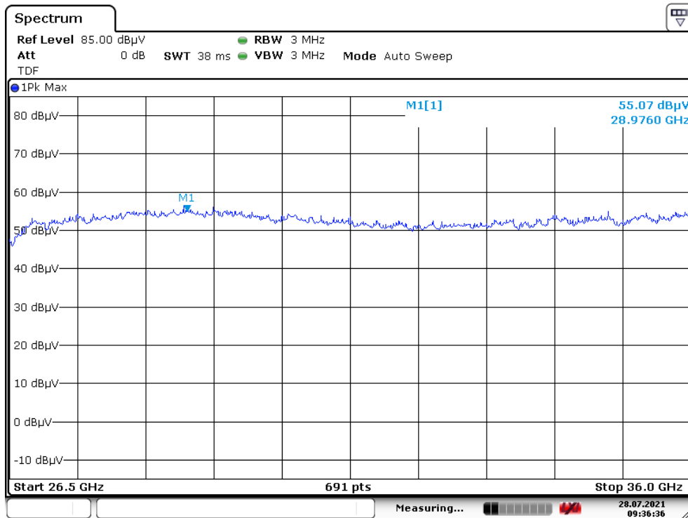
Plot 16: Pre-scan plot with peak detector Radiated emissions from 26.5 GHz – 36 GHz, 5GHz + BT mode
