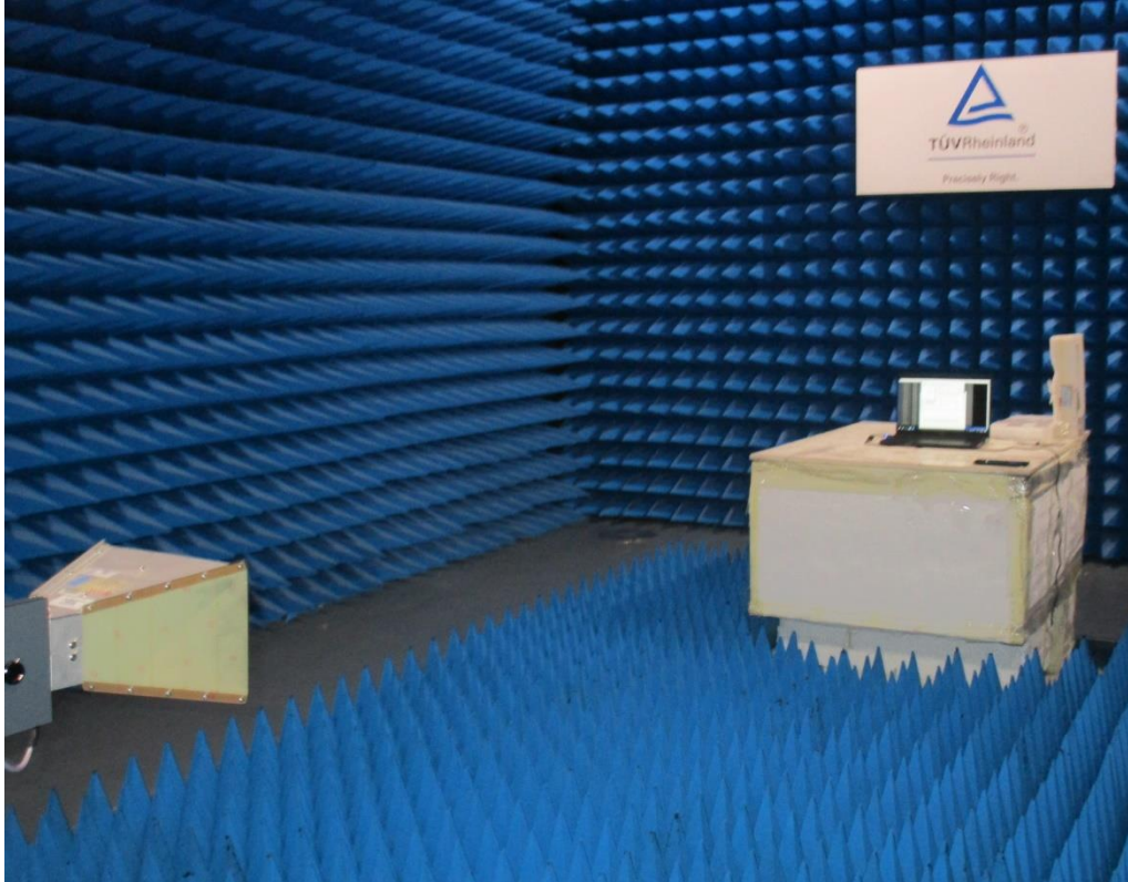
Photo 2: Photograph radiated emissions 1 – 18 GHz
