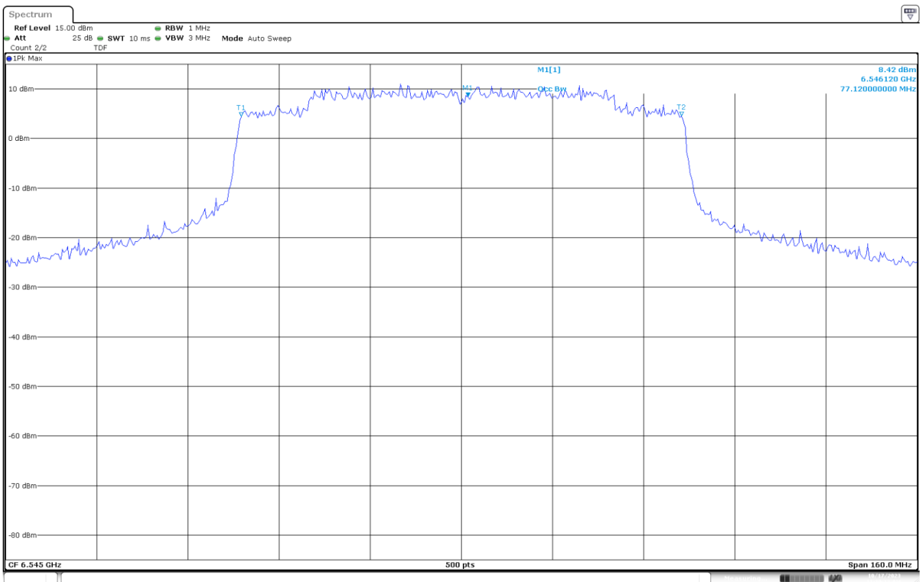
UNII-6 SISO A 802.11ax80 CH119 6545MHz 99%
