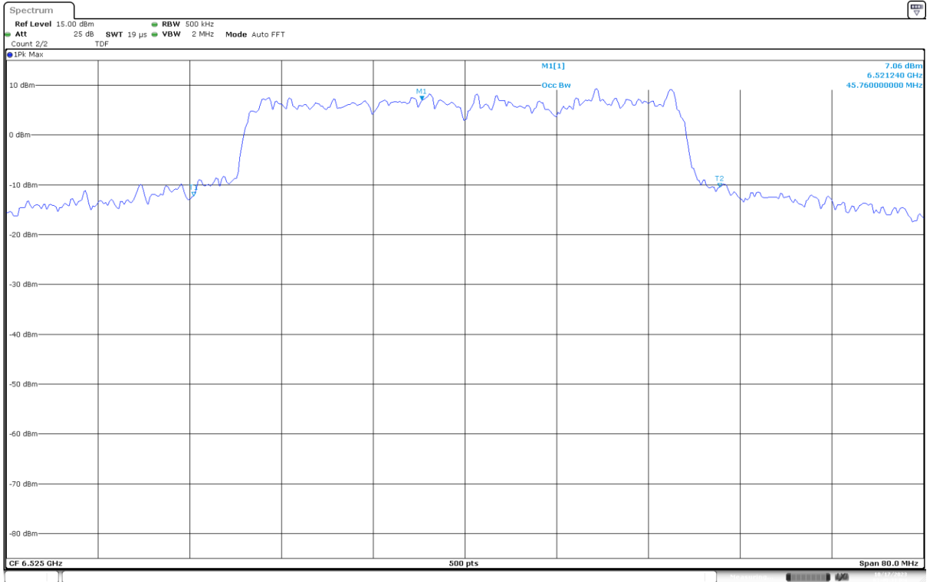
UNII-6 MIMO A 802.11ax40 CH115 6525MHz 99%
