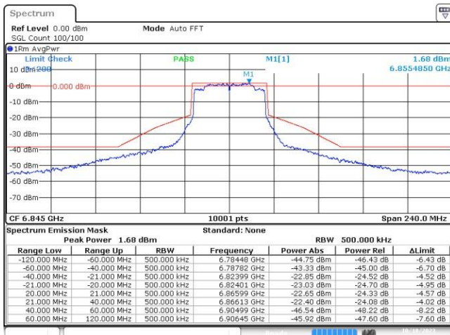
MIMO B-802.11ax-40MHz-Ch179-6845MHz-MCS0
