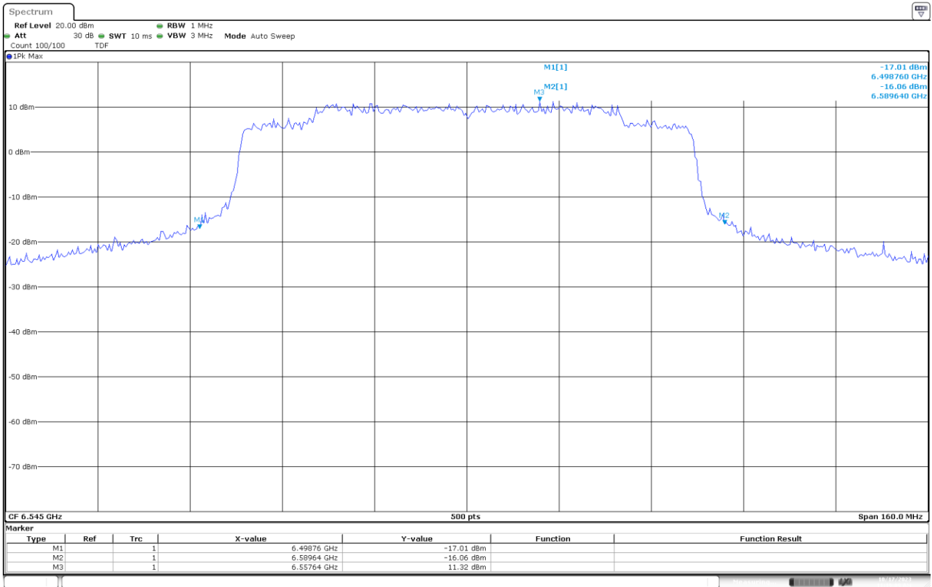
UNII-6 SISO A 802.11ax80 CH119 6545MHz 26dB
