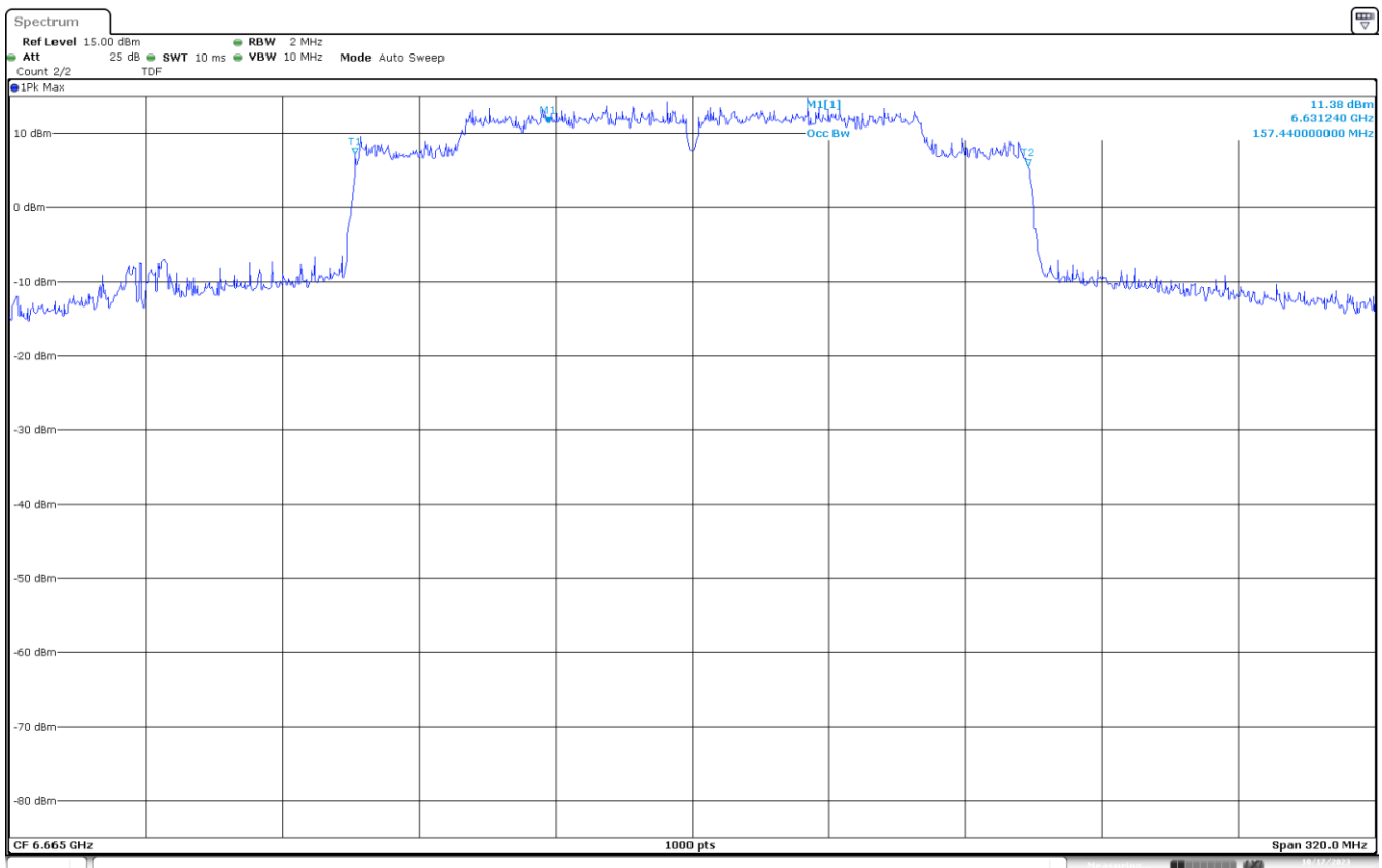
UNII-7 MIMO A 802.11ax160 CH143 6665MHz 99%
