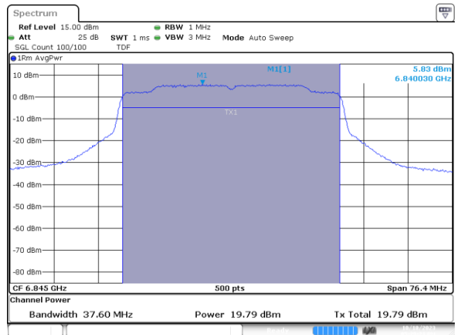
MIMO B-802.11ax-40MHz-Ch179-6845MHz-MCS0
