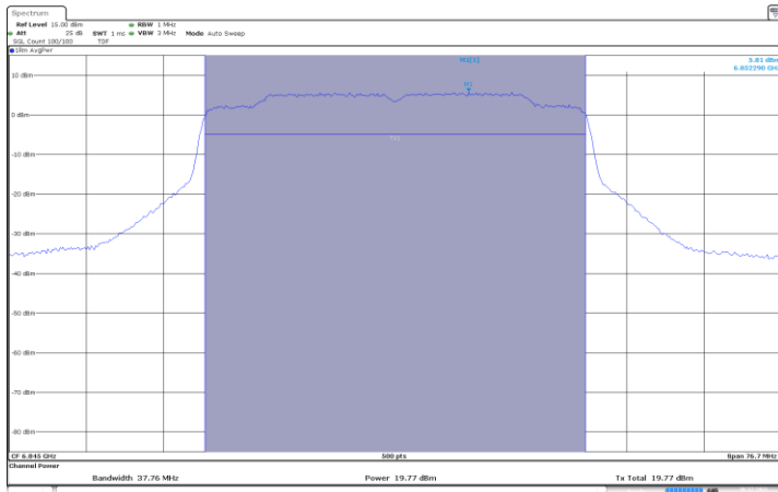
MIMO A-802.11ax-40MHz-Ch179-6845MHz-MCS0
