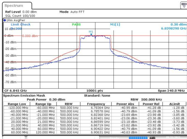
MIMO A-802.11ax-40MHz-Ch179-6845MHz-MCS0
