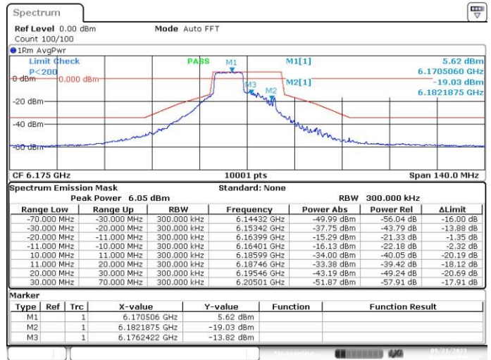
SISO-A, 802.11ax/be20-MCS0, Ch45-8m-53
