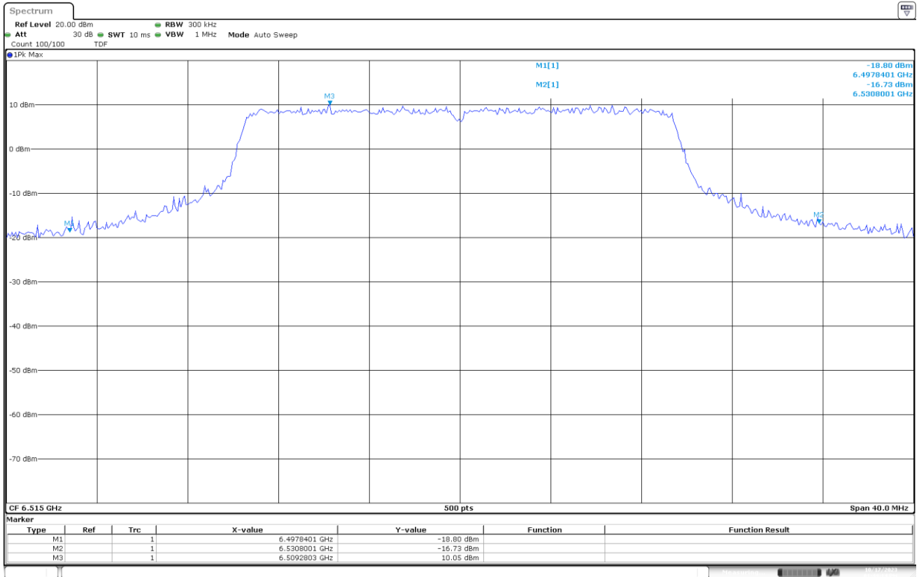
UNII-6 MIMO A 802.11ax20 CH113 6515MHz 26dB
