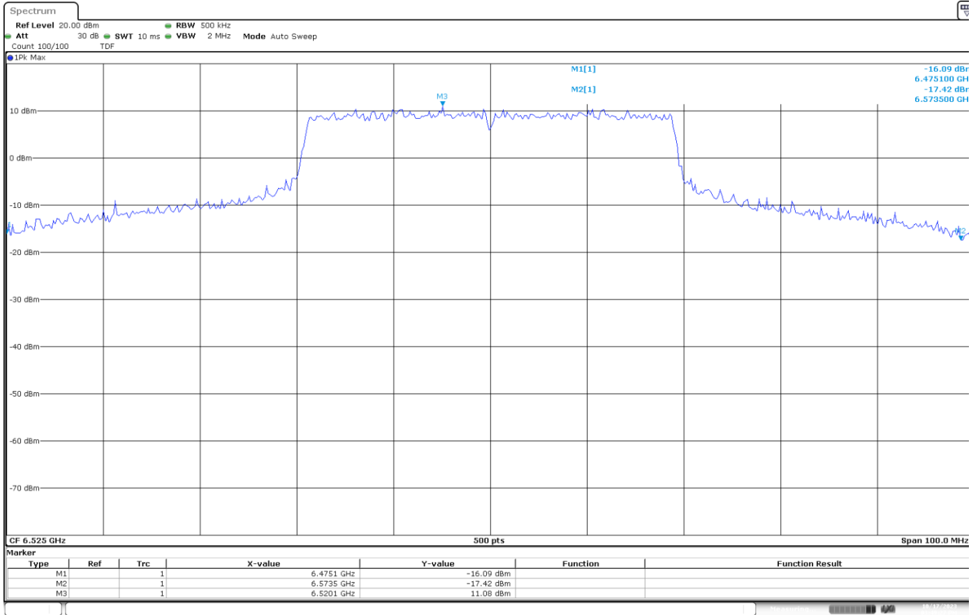
UNII-6 MIMO A 802.11ax40 CH115 6525MHz 26dB
