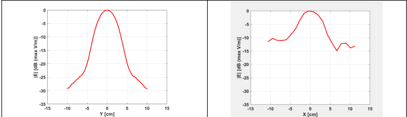
Field variation through the maximum along the H-field polarization
