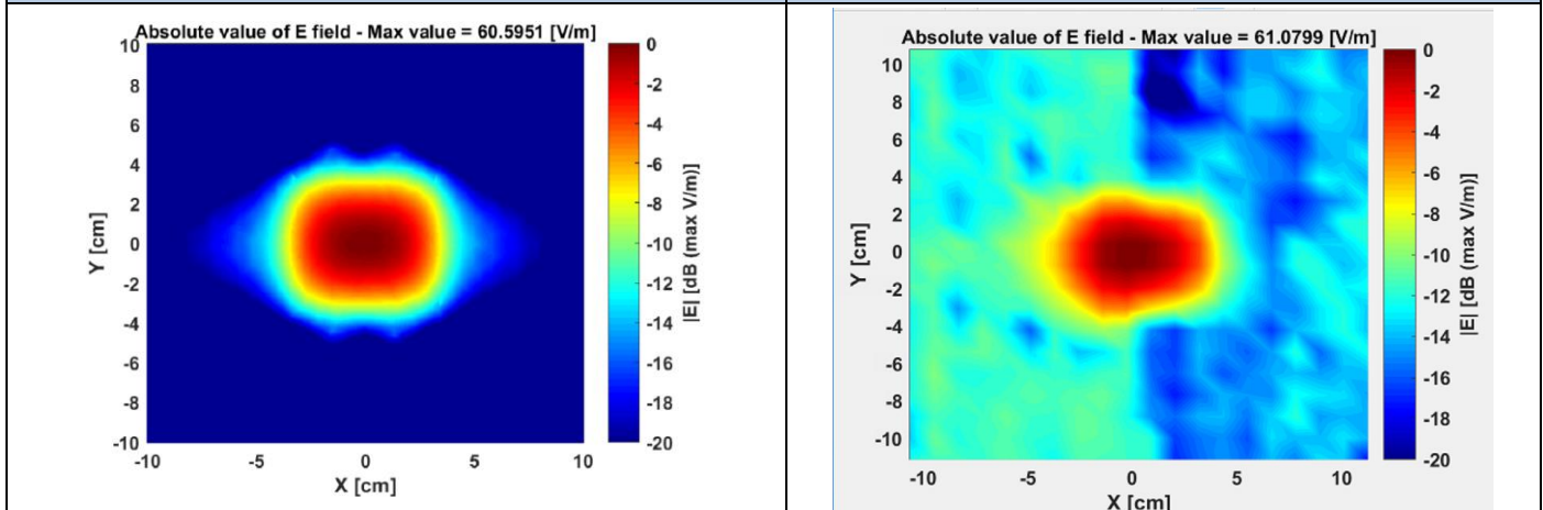
Field variation through the maximum along the E-field polarization
