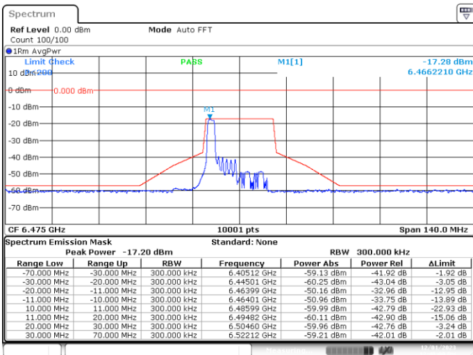
MIMO-B, 802.11ax20-MCS0, Ch105-2m-0
