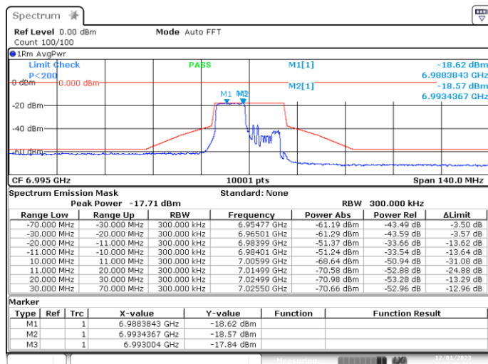
MIMO-A, 802.11ax20-MCS0, Ch209-8m-53
