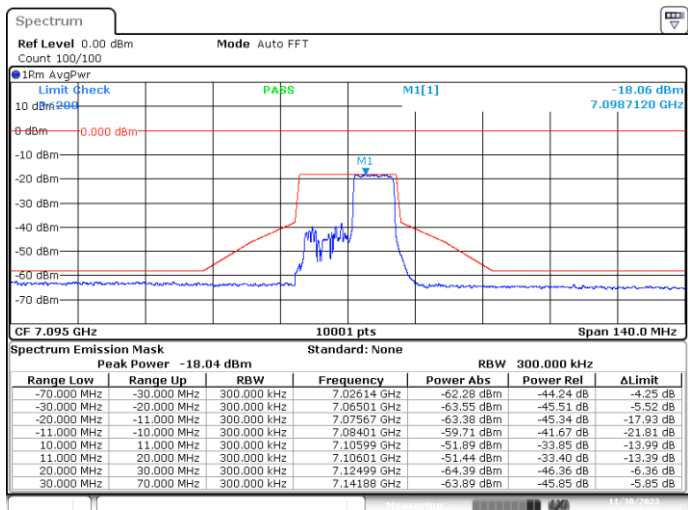
MIMO-A, 802.11ax20-MCS0, Ch229-8m-54
