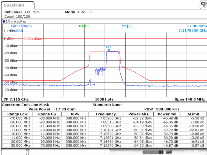
MIMO-A, 802.11ax20-MCS0, Ch233-8m-54
