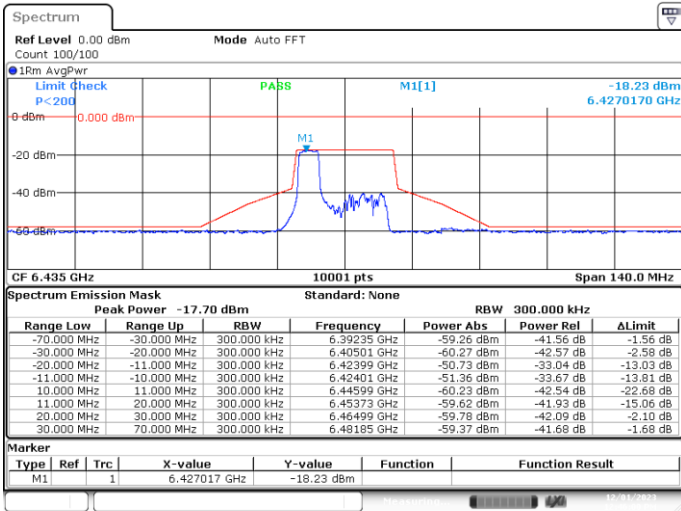
MIMO-B, 802.11ax20-MCS0, Ch97-4m-37
