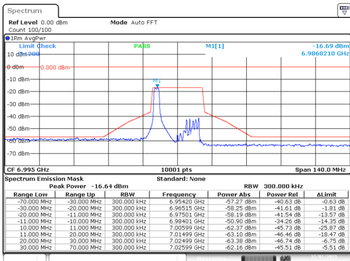
MIMO-A, 802.11ax20-MCS0, Ch209-2m-0
