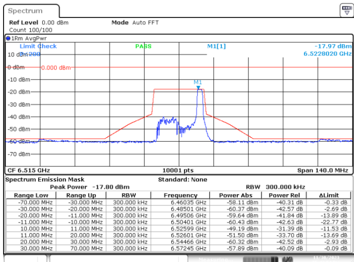
MIMO-A, 802.11ax20-MCS0, Ch113-2m-0
