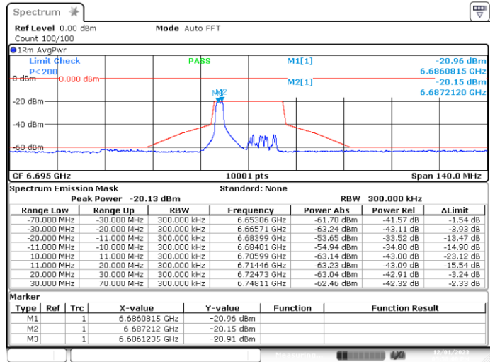
MIMO-A, 802.11ax20-MCS0, Ch149-2m-0
