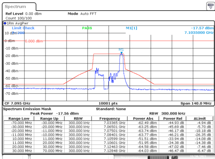
MIMO-A, 802.11ax20-MCS0, Ch229-2m-8
