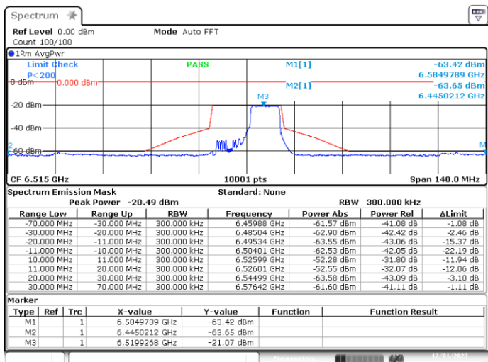
MIMO-A, 802.11ax20-MCS0, Ch113-8m-53
