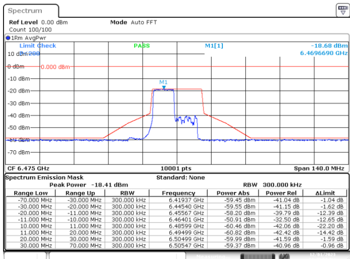
MIMO-B, 802.11ax20-MCS0, Ch105-8m-53
