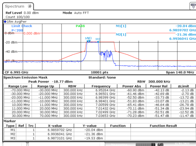
MIMO-B, 802.11ax20-MCS0, Ch209-8m-53
