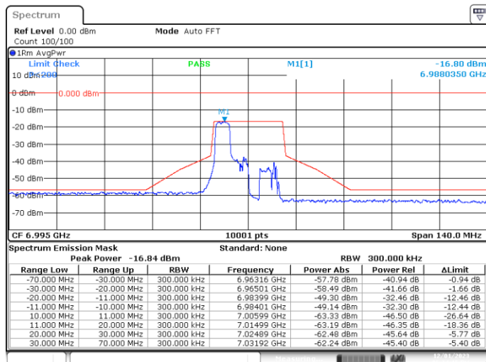
MIMO-A, 802.11ax20-MCS0, Ch209-4m-37
