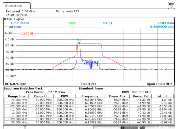
MIMO-A, 802.11ax20-MCS0, Ch185-2m-0
