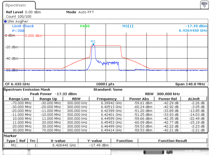
MIMO-B, 802.11ax20-MCS0, Ch97-2m-0
