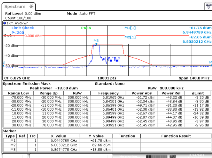
MIMO-A, 802.11ax20-MCS0, Ch185-4m-37
