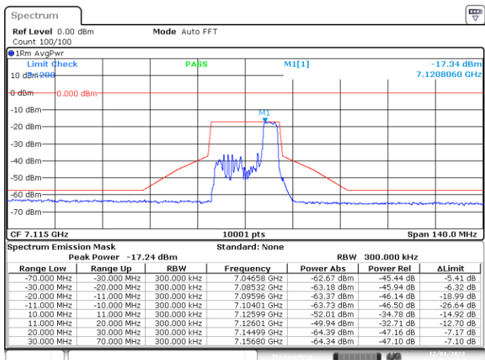
MIMO-A, 802.11ax20-MCS0, Ch233-4m-40
