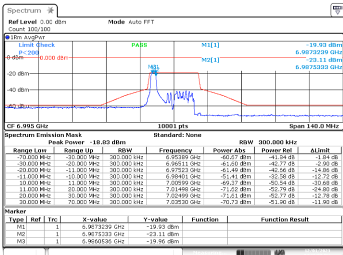
MIMO-B, 802.11ax20-MCS0, Ch209-2m-0
