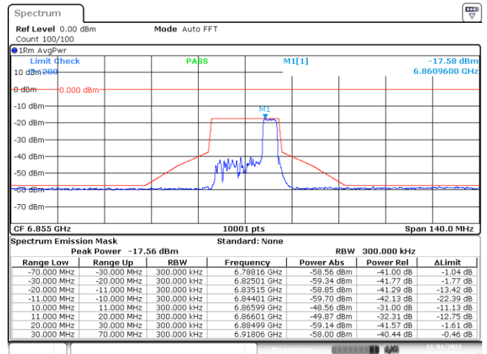
MIMO-A, 802.11ax20-MCS0, Ch181-4m-37
