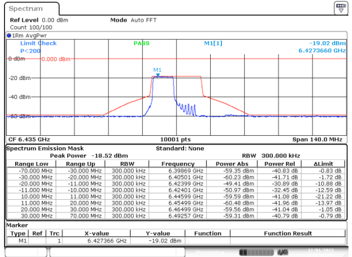
MIMO-B, 802.11ax20-MCS0, Ch97-8m-53
