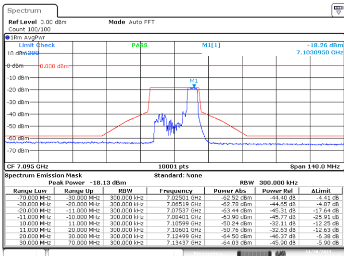
MIMO-A, 802.11ax20-MCS0, Ch229-4m-40
