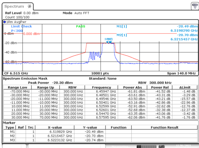
MIMO-B, 802.11ax20-MCS0, Ch113-8m-53
