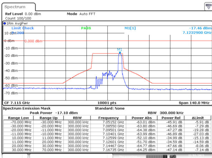
MIMO-A, 802.11ax20-MCS0, Ch233-2m-8
