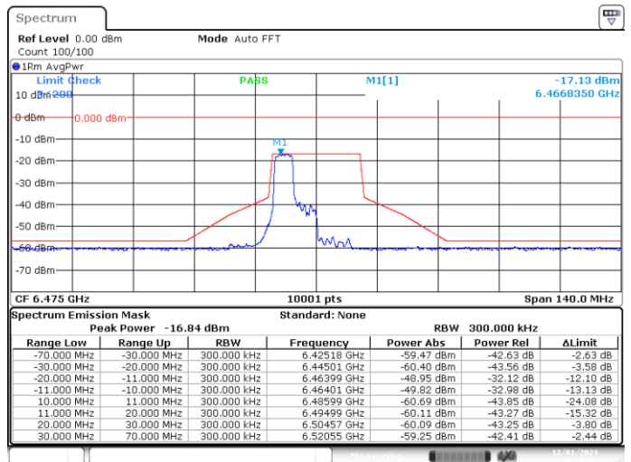
MIMO-B, 802.11ax20-MCS0, Ch105-4m-37
