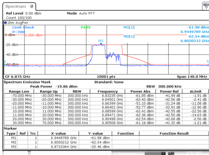
MIMO-B, 802.11ax20-MCS0, Ch185-8m-53
