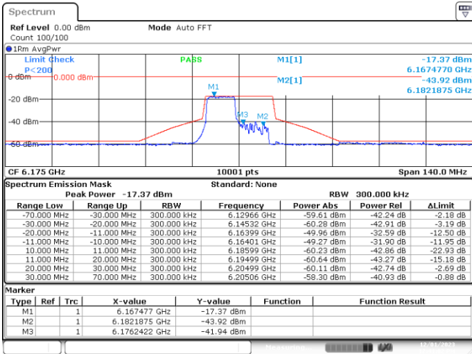
MIMO-B, 802.11ax20-MCS0, Ch45-8m-53
