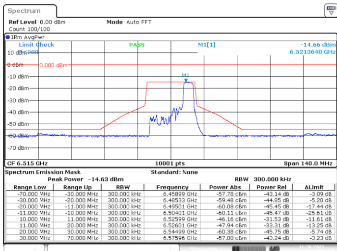
SISO-B, 802.11ax20-MCS0, Ch113-4m-37
