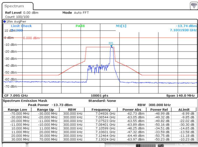
SISO-A, 802.11ax20-MCS0, Ch229-2m-8
