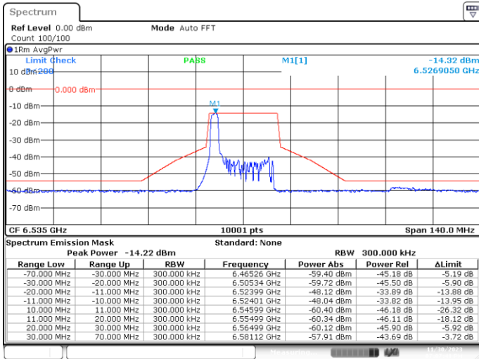
SISO-B, 802.11ax20-MCS0, Ch117-2m-0
