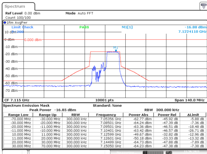
SISO-B, 802.11ax20-MCS0, Ch233-8m-54
