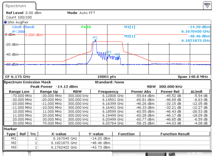
SISO-B, 802.11ax20-MCS0, Ch45-2m-0
