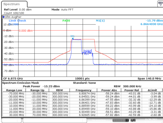
SISO-A, 802.11ax20-MCS0, Ch185-8m-53
