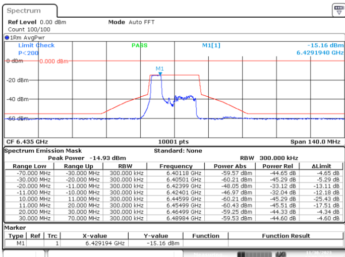
SISO-B, 802.11ax20-MCS0, Ch97-4m-37
