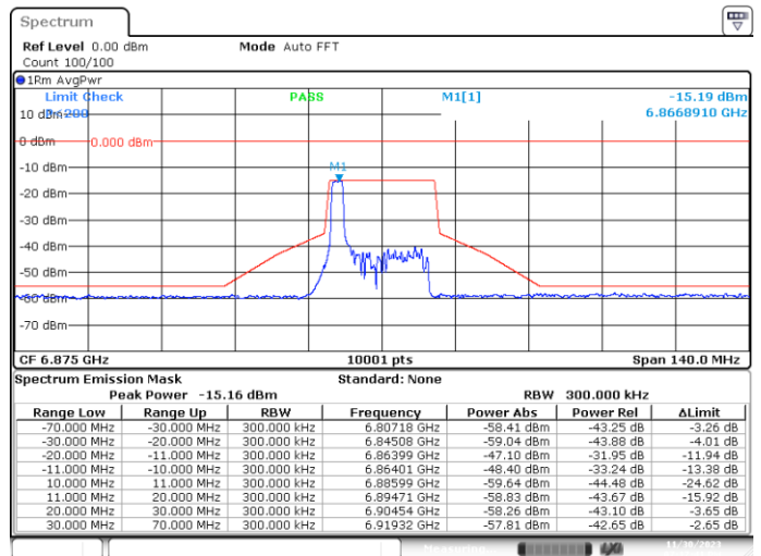
SISO-B, 802.11ax20-MCS0, Ch185-2m-0
