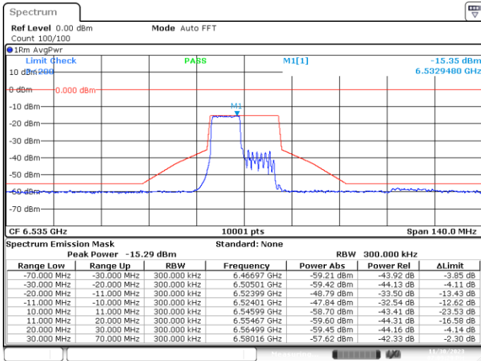
SISO-B, 802.11ax20-MCS0, Ch117-8m-53
