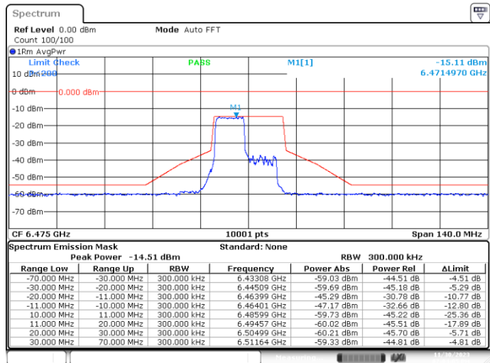
SISO-B, 802.11ax20-MCS0, Ch105-8m-53
