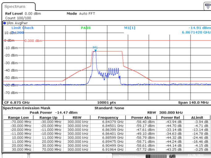
SISO-A, 802.11ax20-MCS0, Ch185-2m-0
