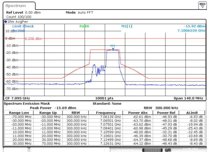
SISO-B, 802.11ax20-MCS0, Ch229-8m-54
