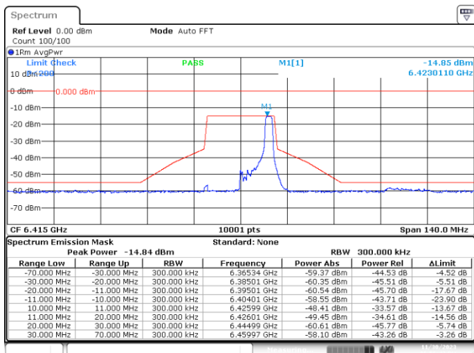
SISO-B, 802.11ax20-MCS0, Ch93-2m-0
