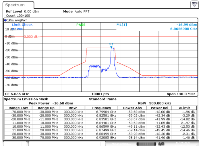
SISO-A, 802.11ax20-MCS0, Ch181-2m-0
