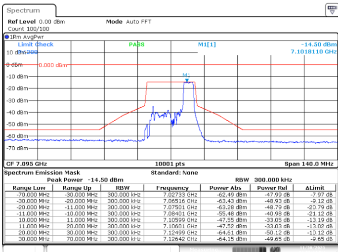
SISO-A, 802.11ax20-MCS0, Ch229-4m-40
