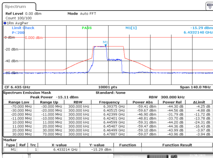
SISO-B, 802.11ax20-MCS0, Ch97-8m-53
