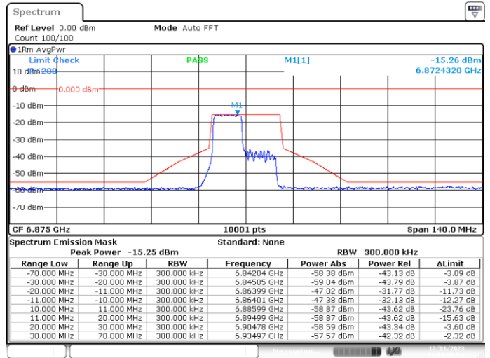
SISO-B, 802.11ax20-MCS0, Ch185-8m-53
