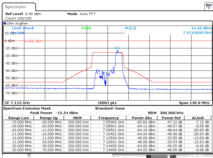
SISO-A, 802.11ax20-MCS0, Ch233-4m-40
