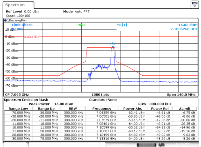
SISO-B, 802.11ax20-MCS0, Ch229-2m-8
