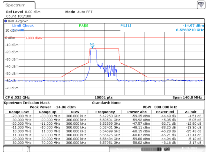
SISO-B, 802.11ax20-MCS0, Ch117-4m-37
