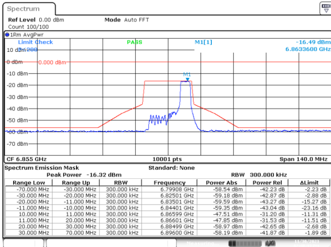
SISO-A, 802.11ax20-MCS0, Ch181-4m-37
