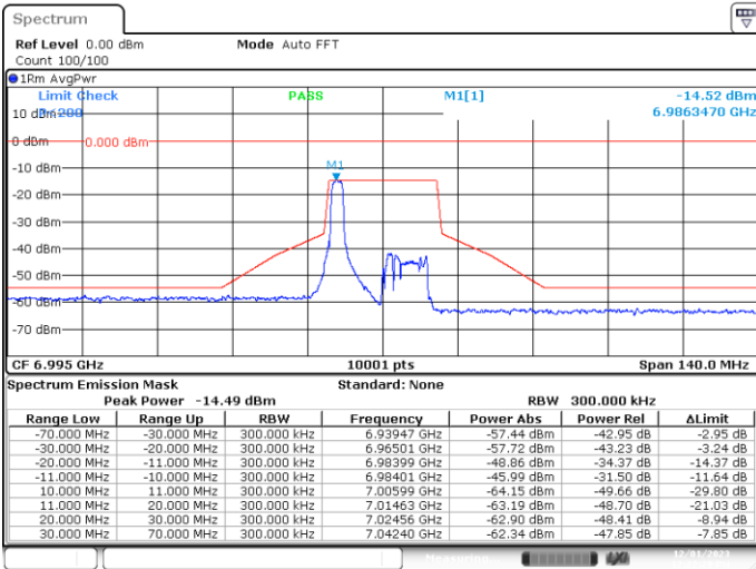
SISO-B, 802.11ax20-MCS0, Ch209-2m-0
