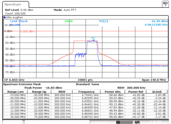
SISO-A, 802.11ax20-MCS0, Ch181-8m-53
