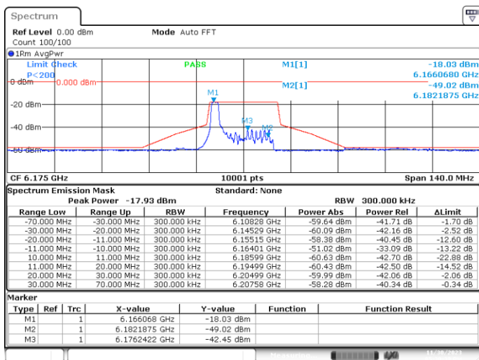
MIMO-A, 802.11ax20-MCS0, Ch45-2m-0
