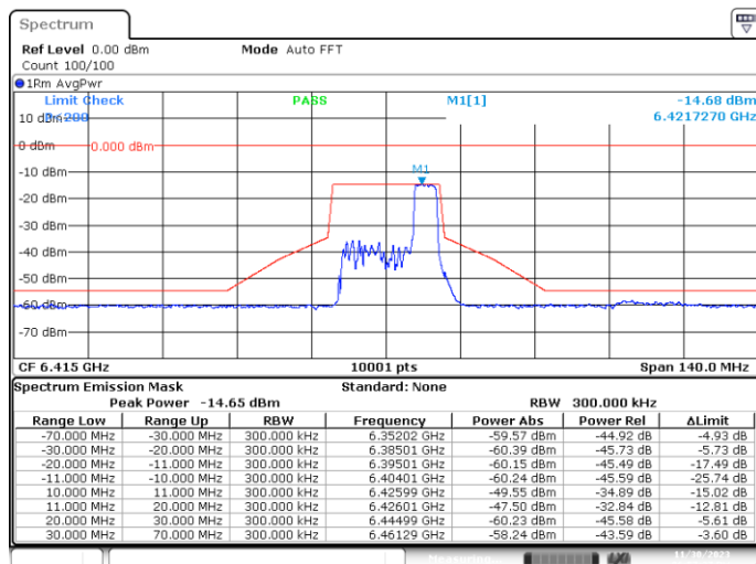
SISO-B, 802.11ax20-MCS0, Ch93-4m-37
