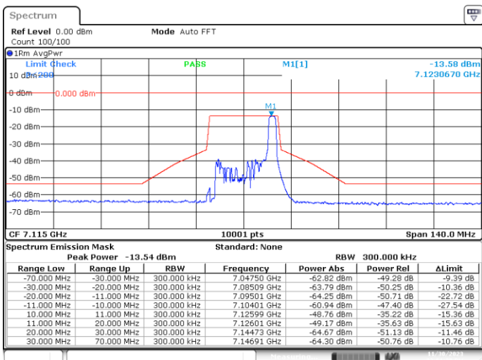
SISO-A, 802.11ax20-MCS0, Ch233-2m-8
