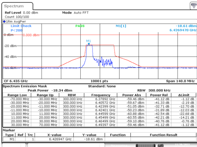
MIMO-A, 802.11ax20-MCS0, Ch97-4m-37
