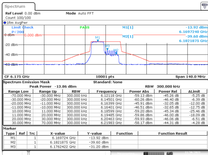
SISO-B, 802.11ax20-MCS0, Ch45-8m-53
