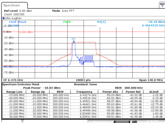
MIMO-A, 802.11ax20-MCS0, Ch105-2m-0
