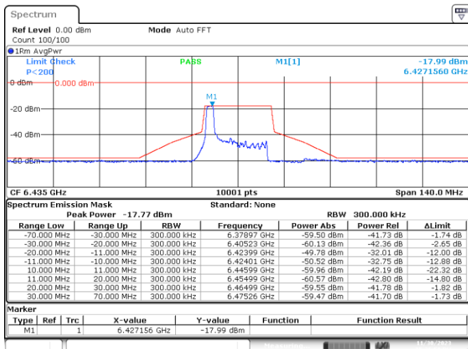
MIMO-A, 802.11ax20-MCS0, Ch97-2m-0
