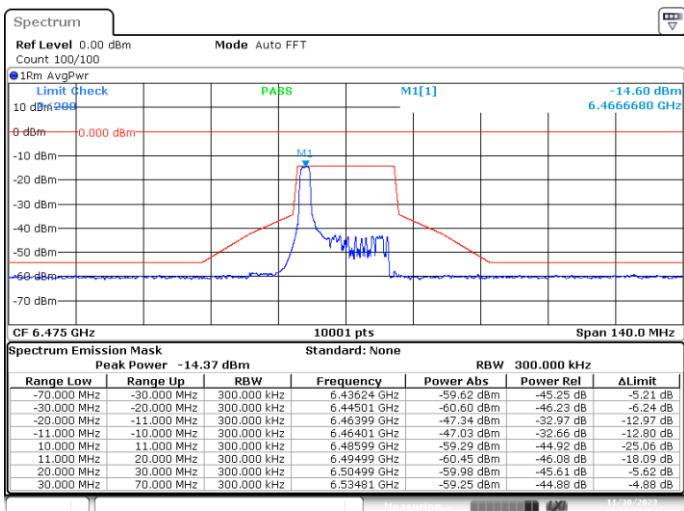
SISO-B, 802.11ax20-MCS0, Ch105-2m-0
