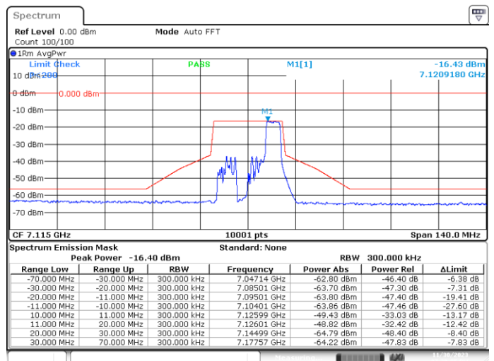
SISO-B, 802.11ax20-MCS0, Ch233-4m-40
