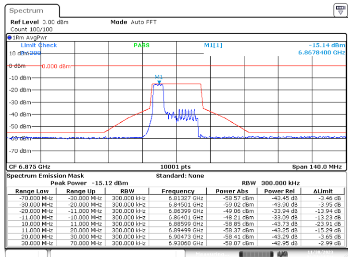
SISO-A, 802.11ax20-MCS0, Ch185-4m-37
