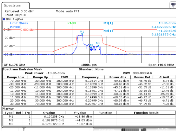
SISO-B, 802.11ax20-MCS0, Ch45-4m-37
