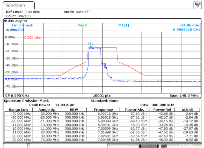
SISO-A, 802.11ax20-MCS0, Ch209-8m-53
