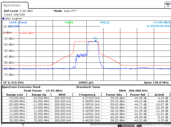
SISO-B, 802.11ax20-MCS0, Ch93-8m-53
