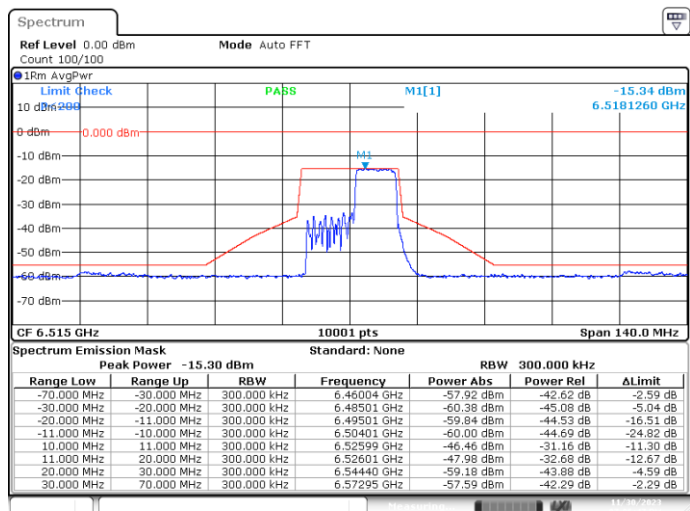
SISO-B, 802.11ax20-MCS0, Ch113-8m-53
