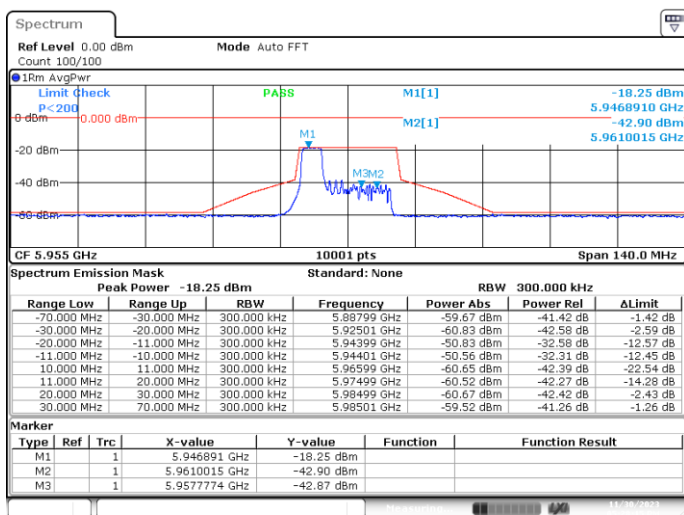
MIMO-A, 802.11ax20-MCS0, Ch1-4m-37
