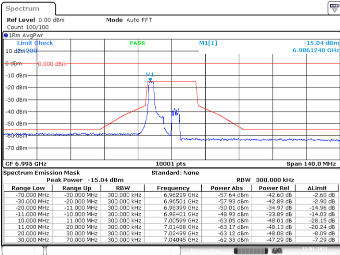
SISO-A, 802.11ax20-MCS0, Ch209-2m-0
