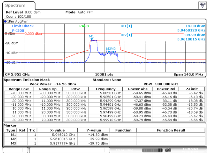
SISO-B, 802.11ax20-MCS0, Ch1-4m-37
