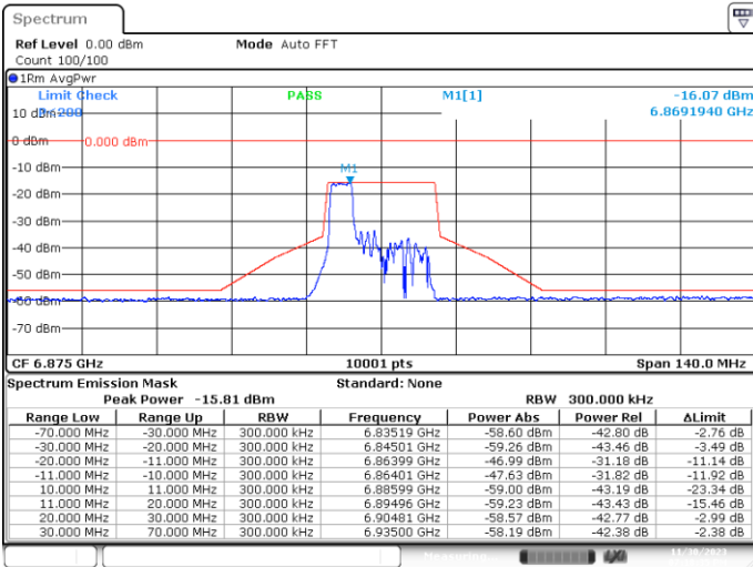
SISO-B, 802.11ax20-MCS0, Ch185-4m-37
