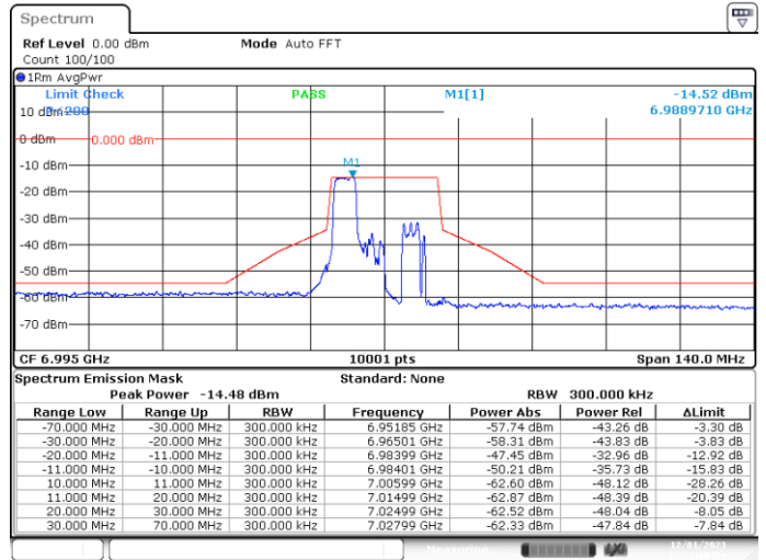
SISO-B, 802.11ax20-MCS0, Ch209-4m-37
