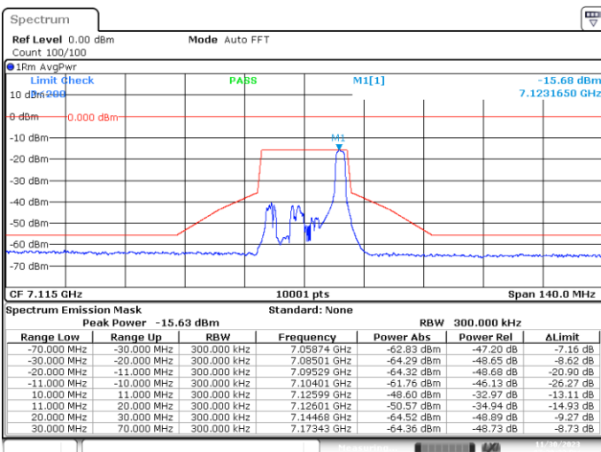
SISO-B, 802.11ax20-MCS0, Ch233-2m-8
