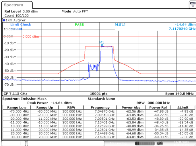
SISO-A, 802.11ax20-MCS0, Ch233-8m-54
