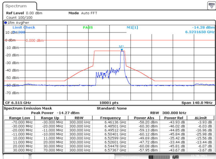
SISO-B, 802.11ax20-MCS0, Ch113-2m-0
