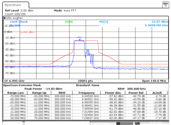
SISO-B, 802.11ax20-MCS0, Ch209-8m-53
