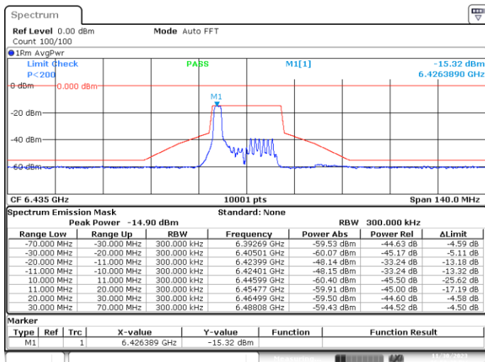
SISO-B, 802.11ax20-MCS0, Ch97-2m-0
