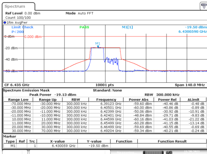
MIMO-A, 802.11ax20-MCS0, Ch97-8m-53
