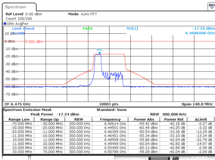
MIMO-A, 802.11ax20-MCS0, Ch105-4m-37
