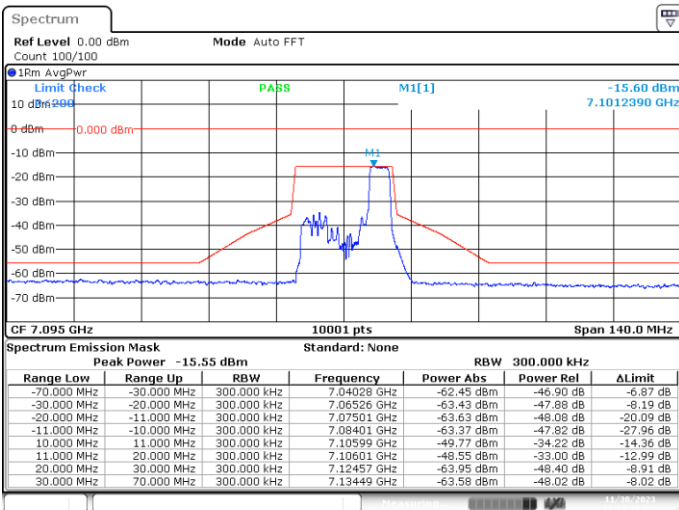
SISO-B, 802.11ax20-MCS0, Ch229-4m-40
