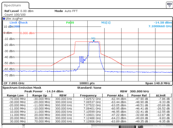
SISO-A, 802.11ax20-MCS0, Ch229-8m-54
