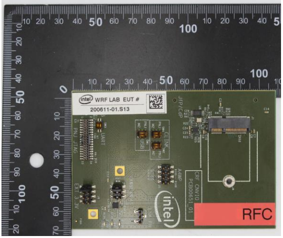
Extender board
