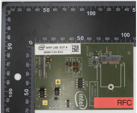
Extender board
