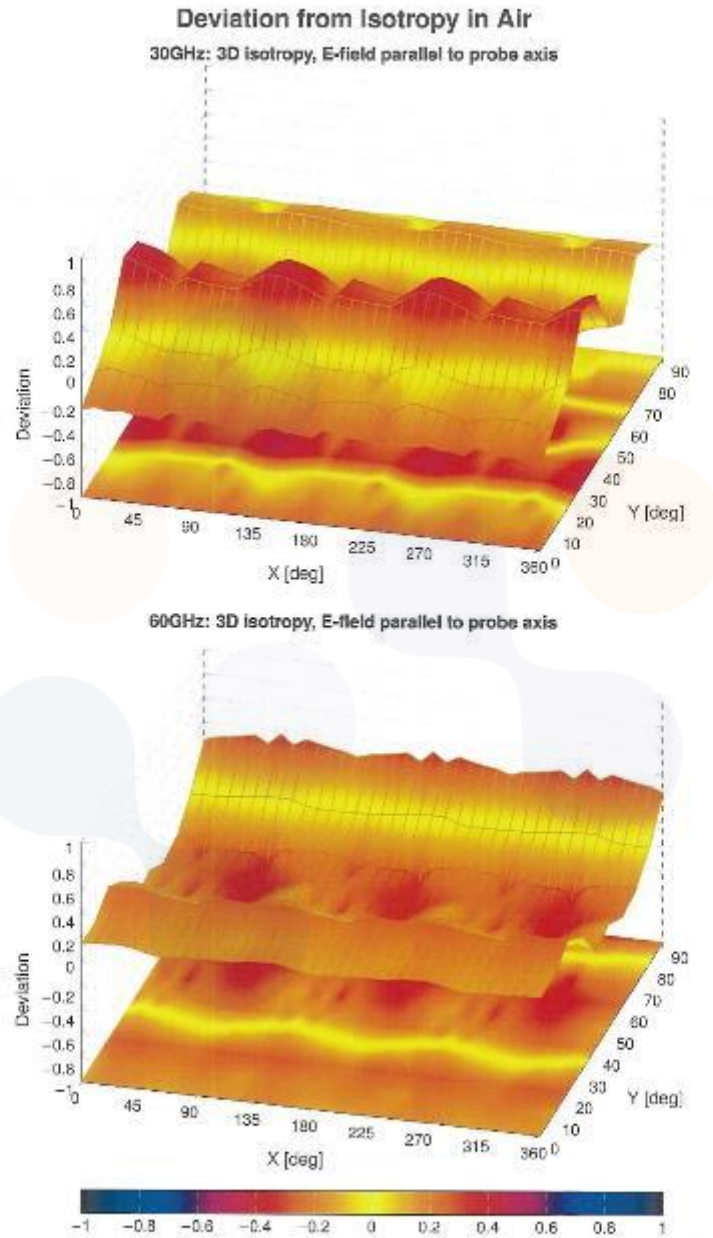
Probe isotropy for E_{\text{rot}} : probe rotated \phi = 0^\circ to 360^\circ , tilted from field propagation direction \vec{k} Parallel to the field propagation ( \psi = 0^\circ - 90^\circ ) at 30 GHz: deviation within \pm 0.47 dB Parallel to the field propagation ( \psi = 0^\circ - 90^\circ ) at 60 GHz: deviation within \pm 0.38 dB
