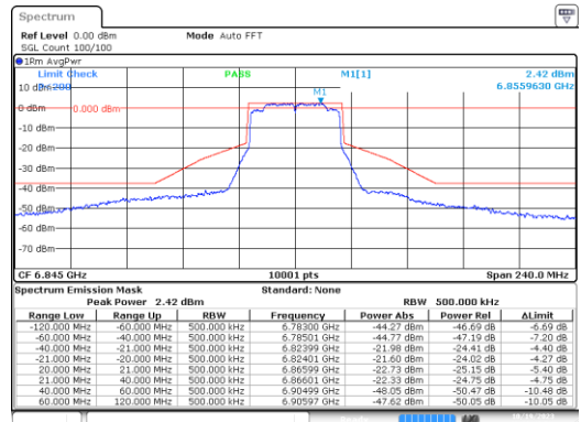
MIMO B-802.11ax-40MHz-Ch179-6845MHz-MCS0
