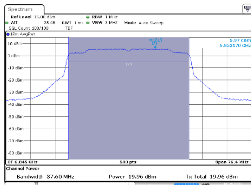
MIMO B-802.11ax-40MHz-Ch179-6845MHz-MCS0
