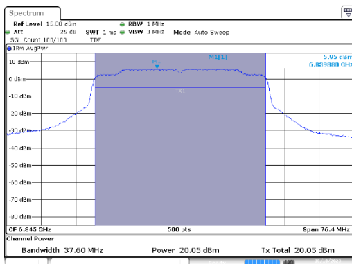
MIMO A-802.11ax-40MHz-Ch179-6845MHz-MCS0
