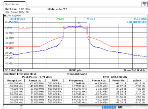
MIMO A-802.11ax-40MHz-Ch179-6845MHz-MCS0
