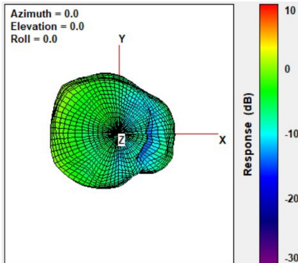
Max Antenna 3D Radiation Pattern 5150-5250 MHz
