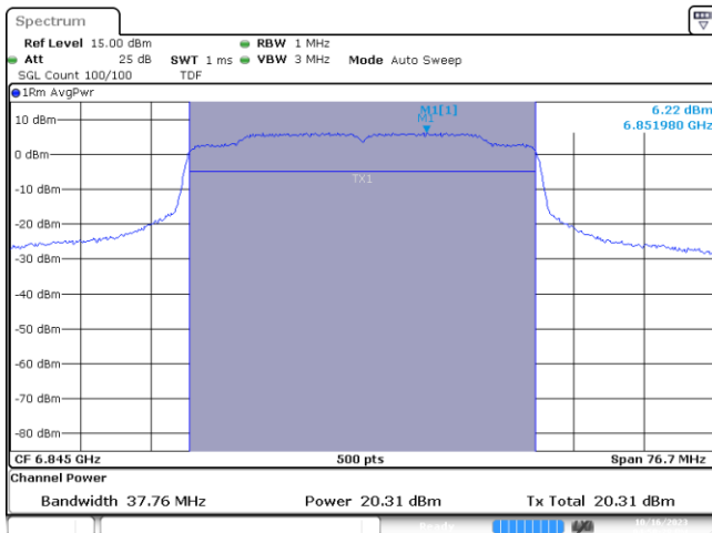
MIMO A-802.11ax-40MHz-Ch179-6845MHz-MCS0
