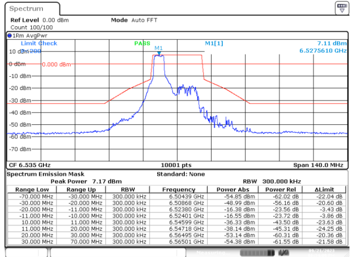
SISO-A, 802.11ax20-MCS0, Ch117-4m-37
