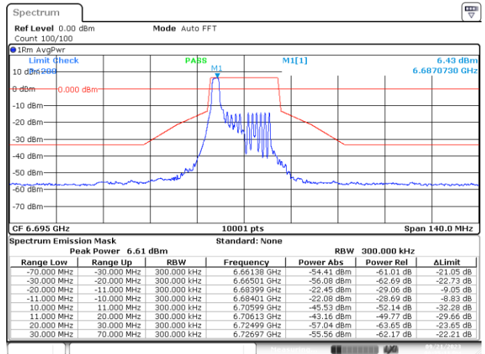
SISO-A, 802.11ax20-MCS0, Ch149-2m-0
