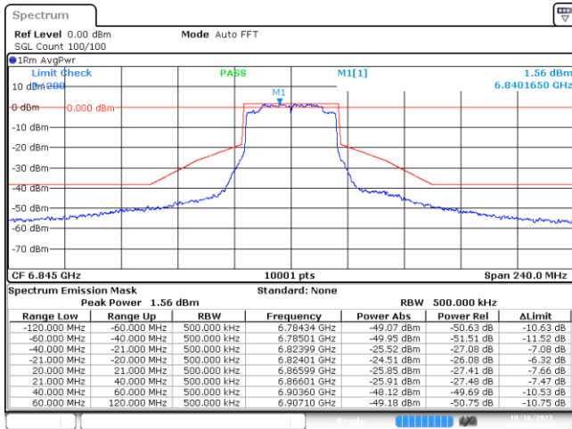
MIMO A-802.11ax-40MHz-Ch179-6845MHz-MCS0
