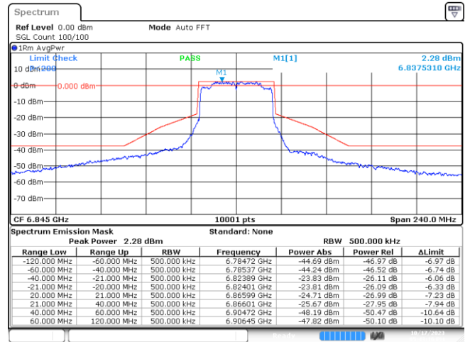
MIMO B-802.11ax-40MHz-Ch179-6845MHz-MCS0
