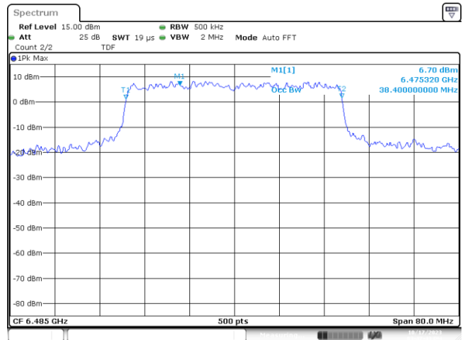
UNII-6 MIMO B 802.11ax40 CH107 6485MHz 99%
