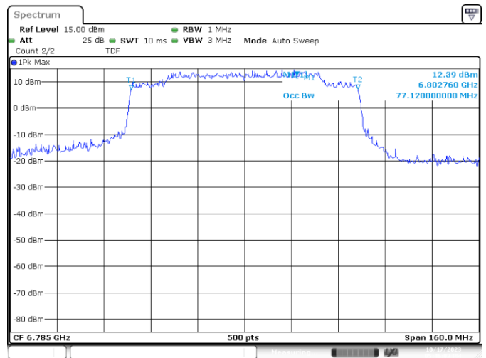
UNII-7 SISO B 802.11ax80 CH167 6785MHz 99%
