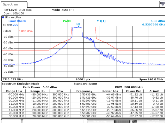
SISO-A, 802.11ax20-MCS0, Ch117-8m-53
