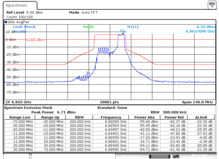
SISO-A, 802.11ax20-MCS0, Ch181-4m-37
