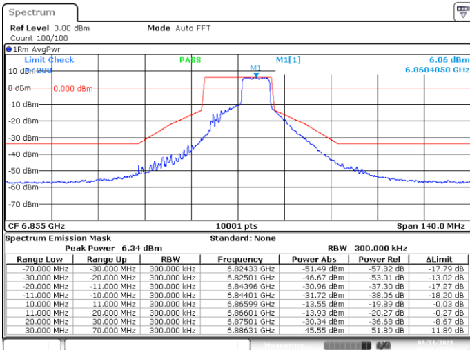
SISO-A, 802.11ax20-MCS0, Ch181-8m-53
