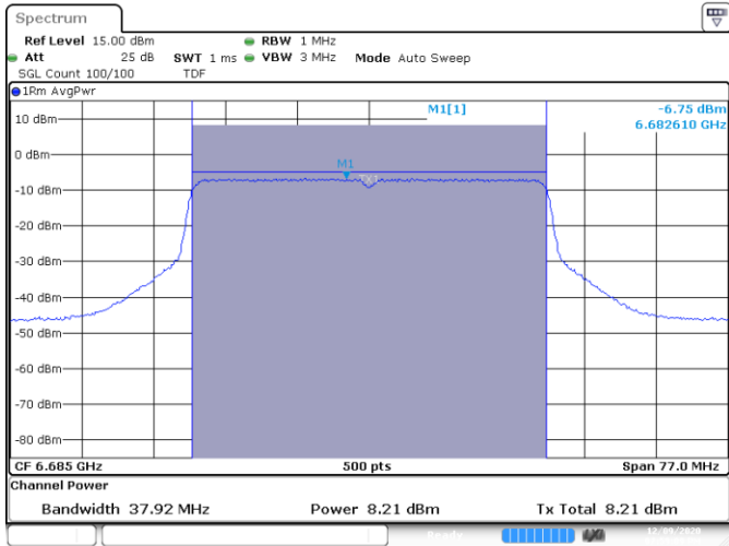
SISO B-802.11ax-40MHz-Ch147-6685MHz-HE0
