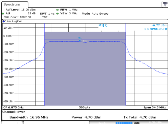
SISO B-802.11a-20MHz-Ch185-6875MHz-6
