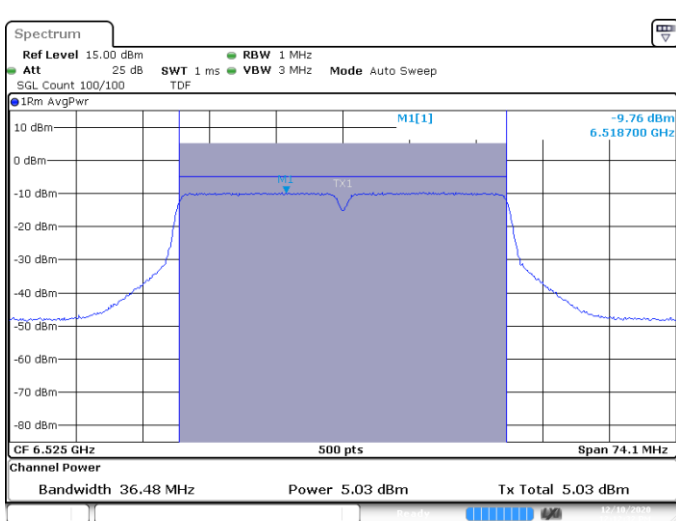
MIMO A-802.11n-40MHz-Ch115-6525MHz-HT8
