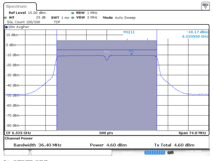
MIMO B-802.11n-40MHz-Ch115-6525MHz-HT8
