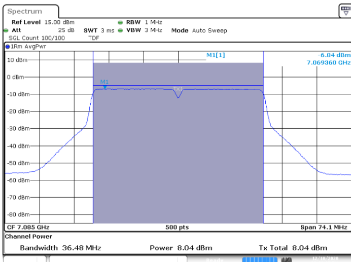
SISO A-802.11n-40MHz-Ch227-7085MHz-HT0
