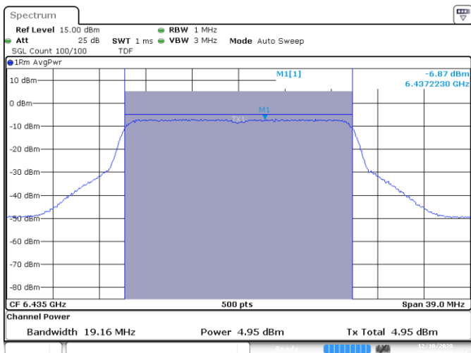
SISO B-802.11ax-20MHz-Ch97-6435MHz-HE0
