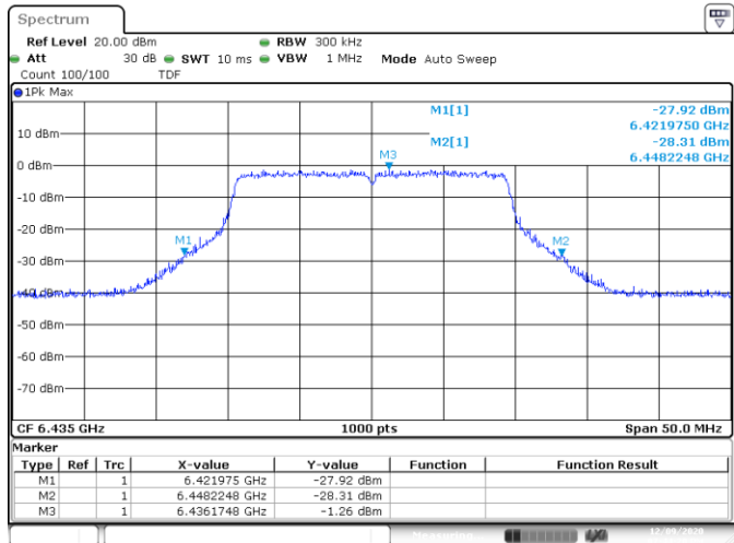
UNII6 SISO B 802.11ax20 ch97 6435MHz 26dB
