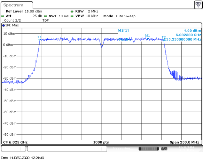
UNII5 SISO A 802.11ac160 ch15 6025MHz 99%
