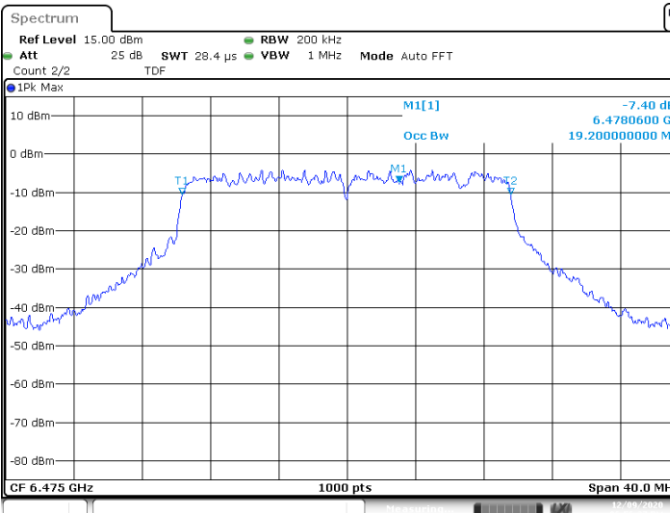
UNII6 SISO A 802.11ax20 ch105 6475MHz 99%
