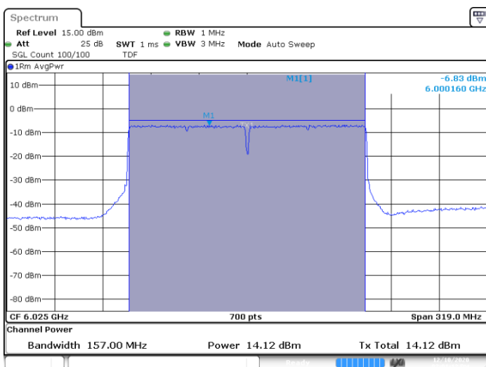
SISO A-802.11ax-160MHz-Ch15-6025MHz-HE0
