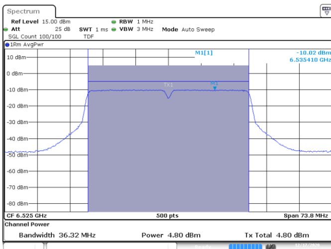
MIMO A-802.11n-40MHz-Ch115-6525MHz-HT8
