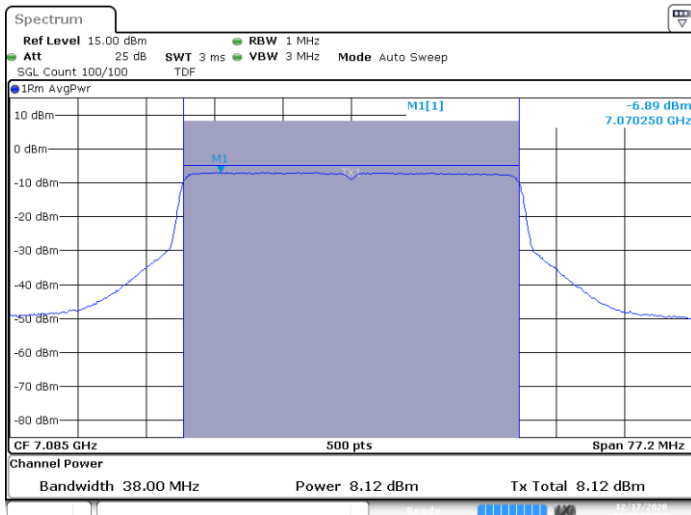
SISO B-802.11ax-40MHz-Ch227-7085MHz-HE0
