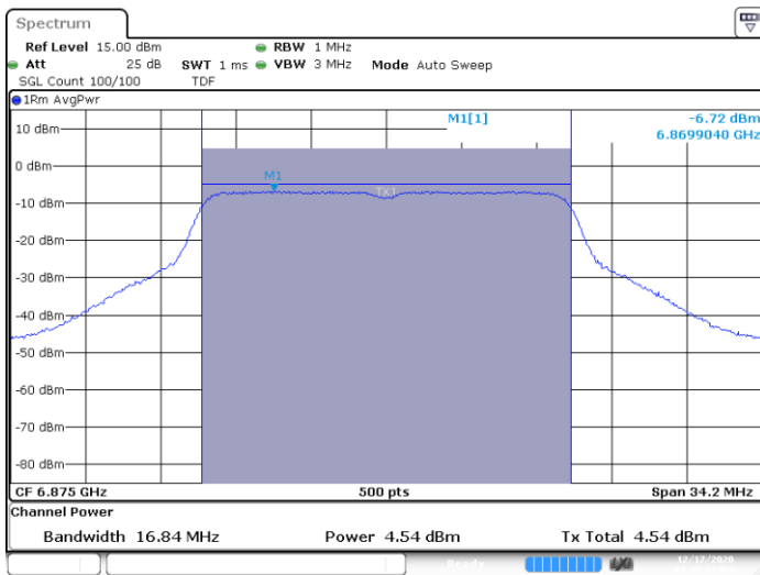
SISO B-802.11a-20MHz-Ch185-6875MHz-6
