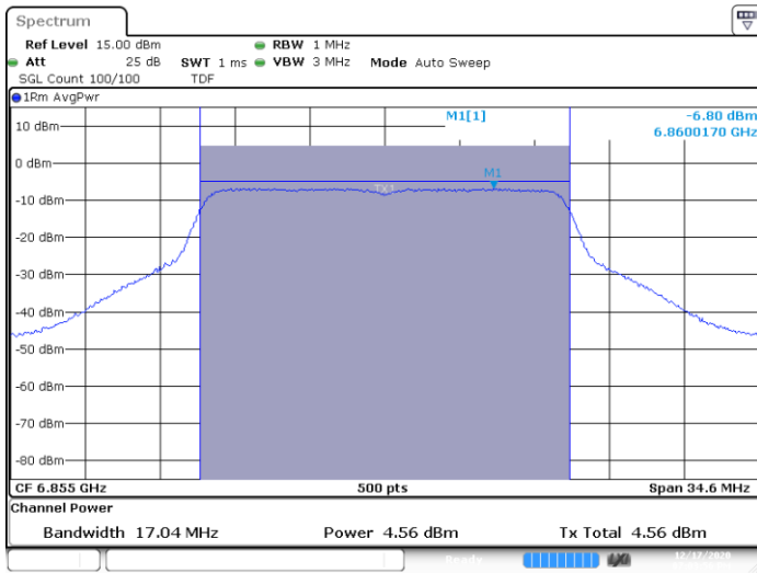
SISO B-802.11a-20MHz-Ch181-6855MHz-6
