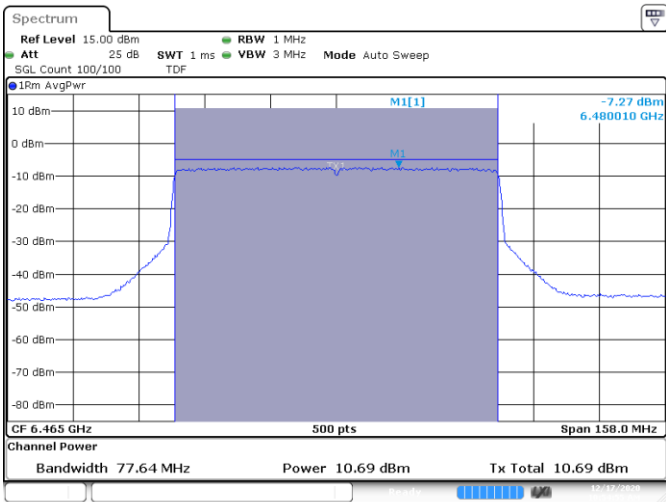
SISO A-802.11ax-80MHz-Ch103-6465MHz-HE0
