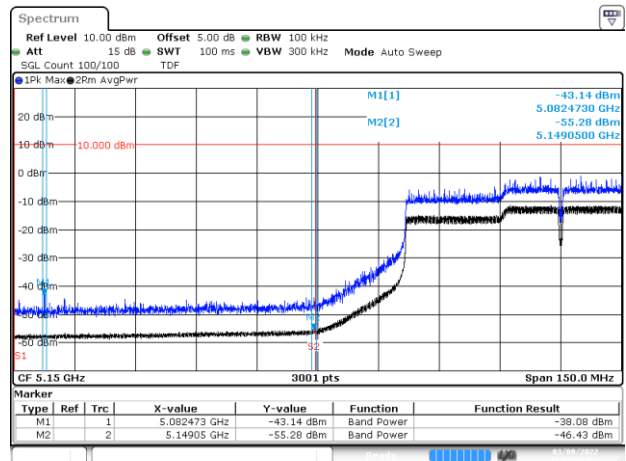
BE-R-LOW, MIMO-B, 802.11ac160-VHT0, Ch50
