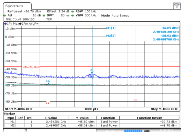
BE-R-HIGH-2MHz, SISO-B, 802.11ax40-HE0, Ch11
