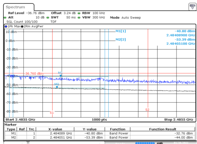
BE-R-HIGH-2MHz, SISO-B, 802.11ax40-HE0, Ch10
