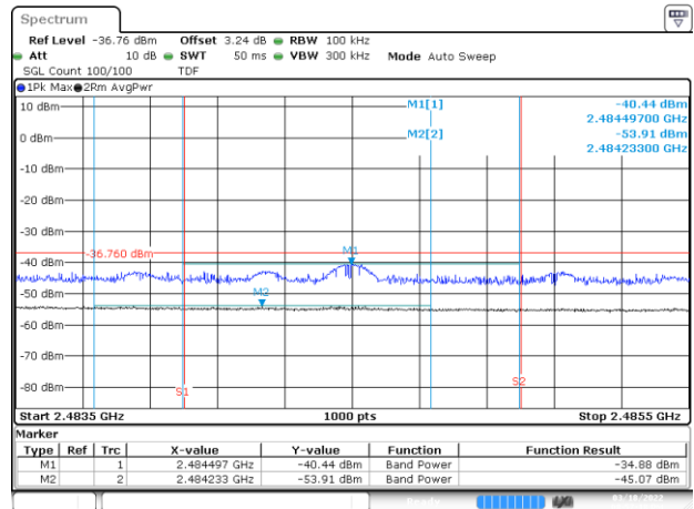
BE-R-HIGH-2MHz, SISO-B, 802.11ax40-HE0, Ch9
