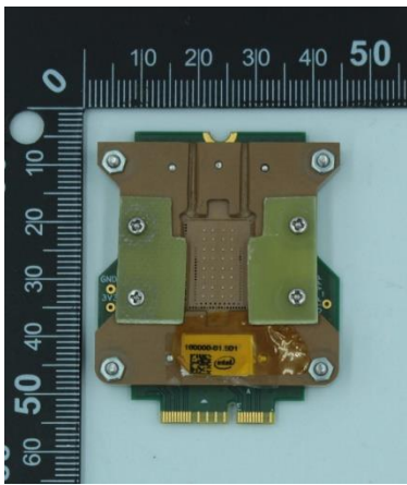
Extender board
