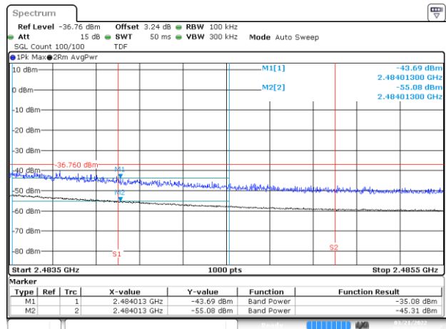
Date: 21.MAR.2022 16:39:21 BE-R-HIGH-2MHz, MIMO-B, 802.11ax20-HE0, Ch12
