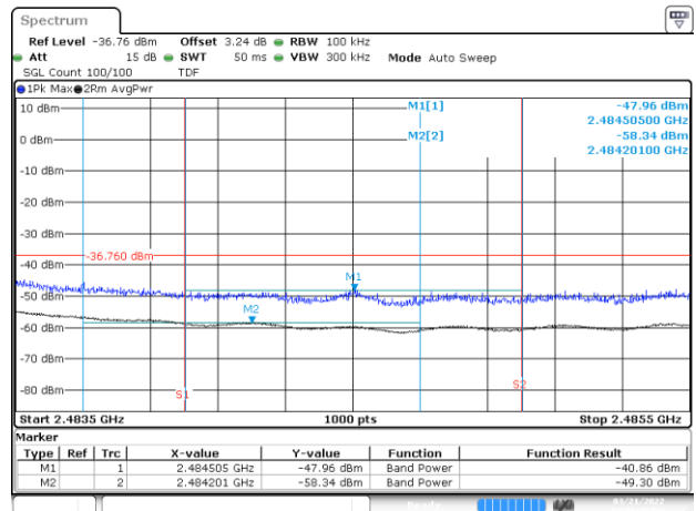
BE-R-HIGH-2MHz, MIMO-B, 802.11n40-HT0, Ch11
