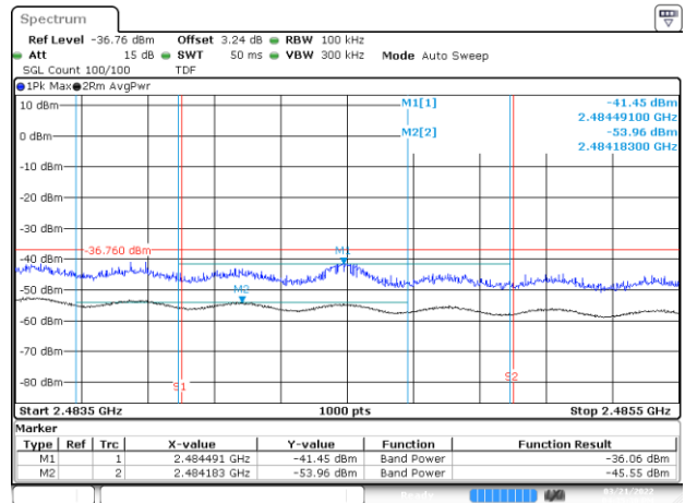
BE-R-HIGH-2MHz, MIMO-B, 802.11n40-HT0, Ch10
