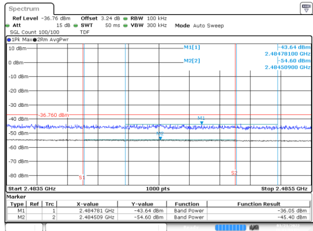
Date: 21.MAR.2022 18:01:04 BE-R-HIGH-2MHz, MIMO-B, 802.11ax20-HE0, Ch11
