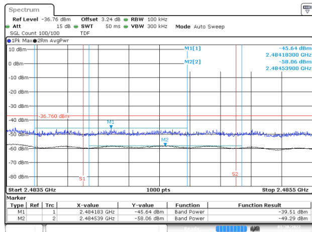
BE-R-HIGH-2MHz, MIMO-A, 802.11n20-HT0, Ch13
