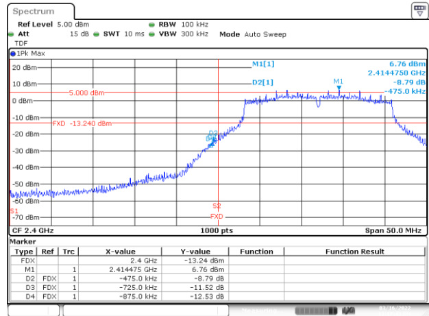
BE-NR, MIMO-B, 802.11n20-HT0, Ch1
