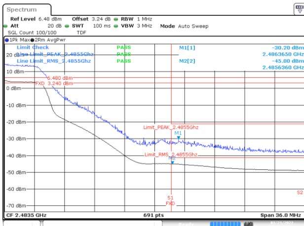
BE-R-HIGH, MIMO-B, 802.11n40-HT0, Ch9
