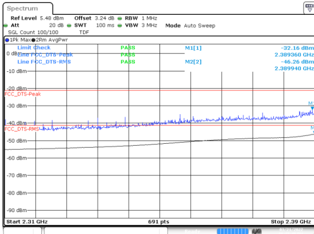
BE-R-LOW, MIMO-B, 802.11n40-HT0, Ch3
