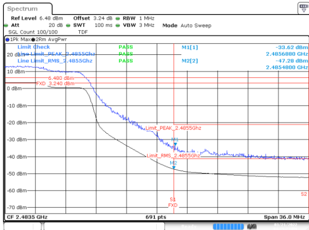
BE-R-HIGH, MIMO-B, 802.11n40-HT0, Ch10
