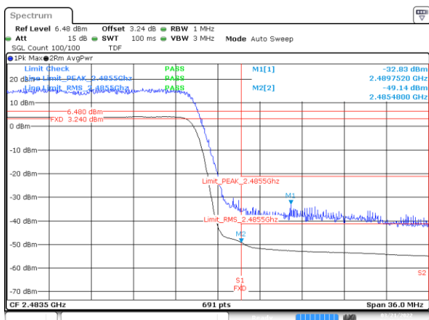
Date: 21.MAR.2022 16:40:31 BE-R-HIGH, MIMO-B, 802.11ax20-HE0, Ch13
