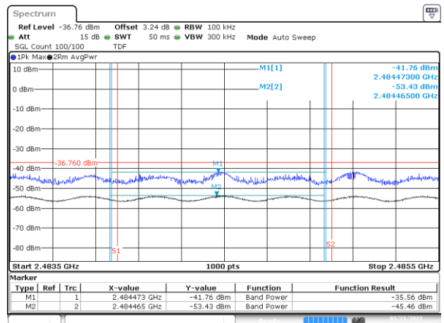
BE-R-HIGH-2MHz, MIMO-B, 802.11n40-HT0, Ch9
