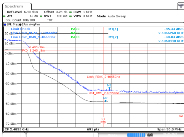
BE-R-HIGH, MIMO-A, 802.11n40-HT0, Ch9
