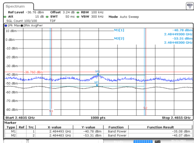
BE-R-HIGH-2MHz, MIMO-B, 802.11n20-HT0, Ch11
