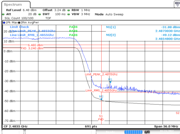
BE-R-HIGH, MIMO-B, 802.11n20-HT0, Ch13
