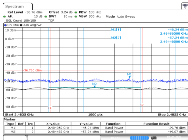
BE-R-HIGH-2MHz, MIMO-A, 802.11n40-HT0, Ch9
