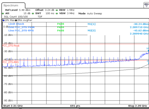
Date 14MAR2022 21:35:55 BE-R-LOW, MIMO-A, 802.11ax20-HE0, Ch1
