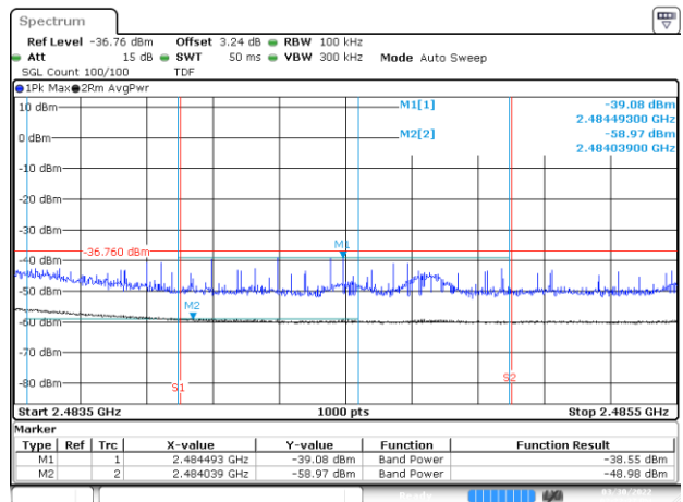
BE-R-HIGH-2MHz, SISO-A, 802.11ax40-HE0, Ch11
