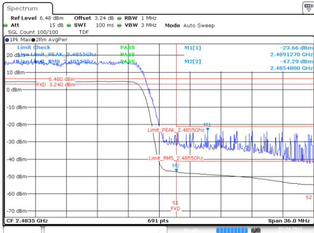
Date 24MAR2022 17:13:14 BE-R-HIGH, SISO-A, 802.11ax20-HE0, Ch13
