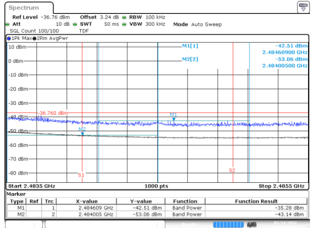
Date 24MAR2022 16:40:31 BE-R-HIGH-2MHz, SISO-A, 802.11ax20-HE0, Ch12
