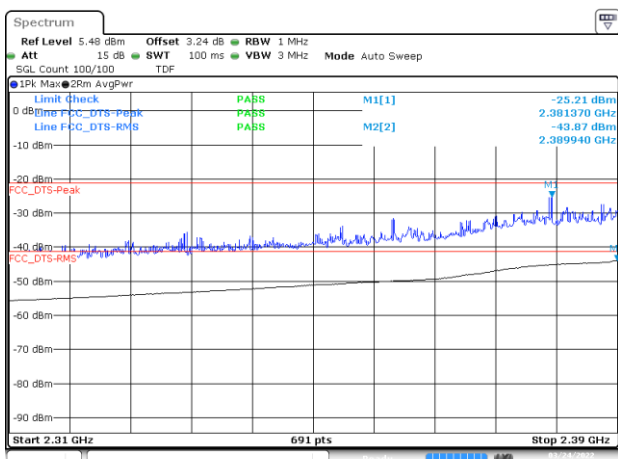
Date 24MAR2022 16:42:52 BE-R-LOW, SISO-A, 802.11ax40-HE0, Ch3
