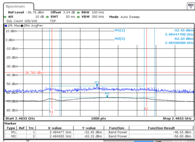
BE-R-HIGH-2MHz, SISO-A, 802.11b-1Mbps, Ch1
