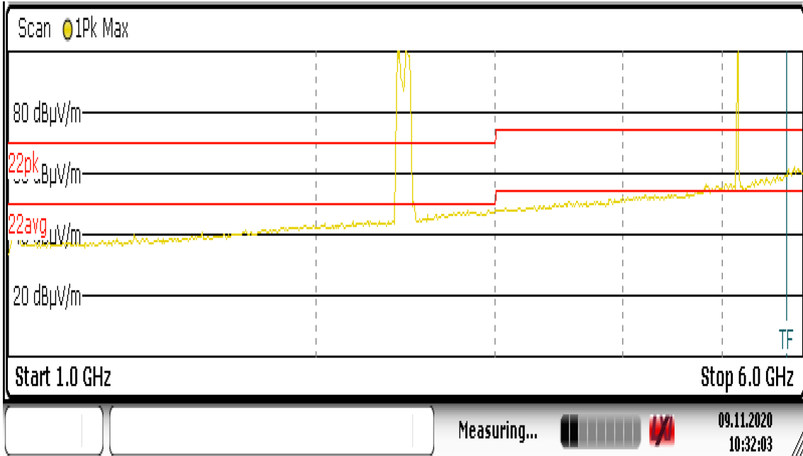
Plot 3: Pre-scan plot with peak detector. Radiated emissions from 1 GHz – 6 GHz, 5GHz + BT mode
