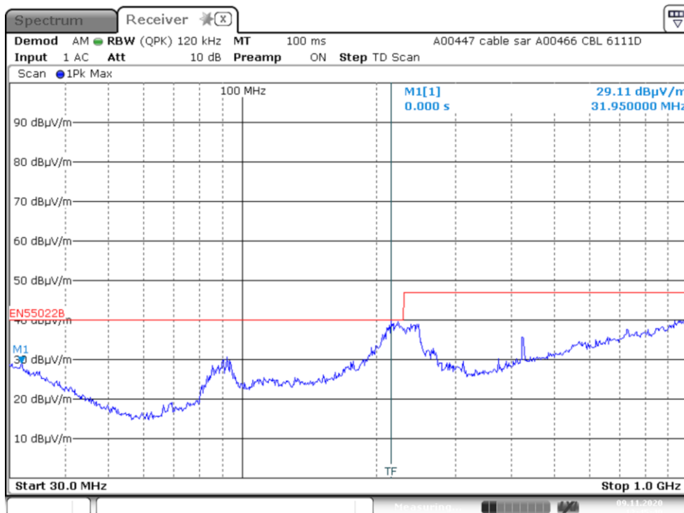
Plot 1: Pre-scan plot with peak detector. Radiated emissions from 30 MHz to 1000 MHz 5GHz + BT mode
