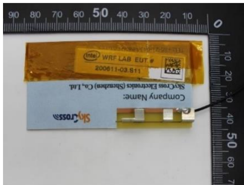
Main Antenna
