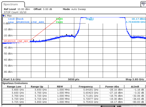
BE-NR-LOW, SISO-B, 802.11ax80-HE0, Ch155
