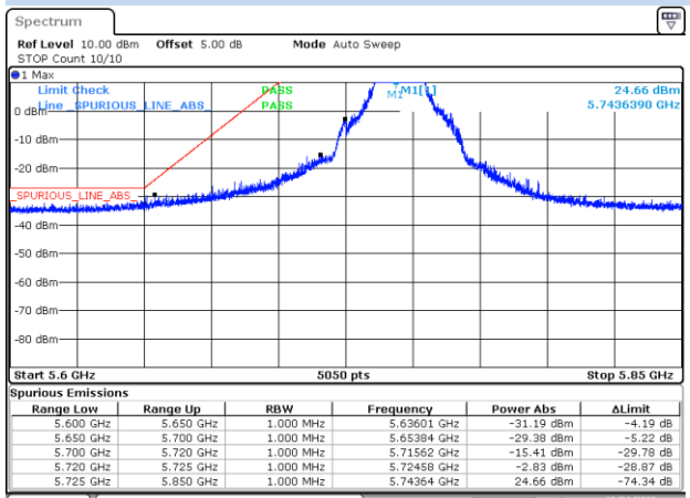
BE-NR-LOW, SISO-B, 802.11a-6Mbps, Ch149
