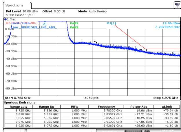
BE-NR-HIGH, SISO-B, 802.11ax80-HE0, Ch155
