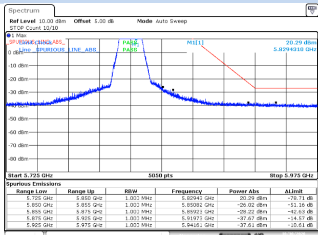
BE-NR-HIGH, MIMO-A, 802.11n20-HT8, Ch165
