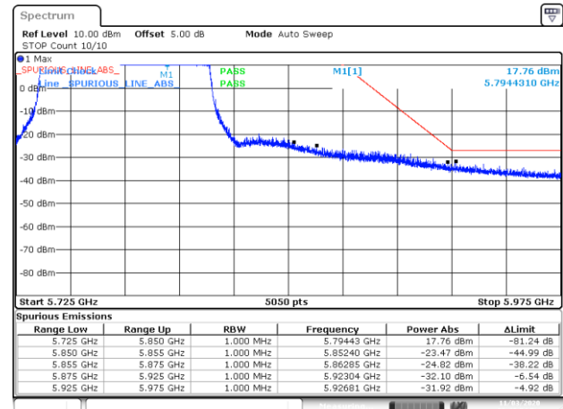
Date: 3 NOV 2020 18:48:55 BE-NR-HIGH, SISO-A, 802.11ax80-HE0, Ch155
