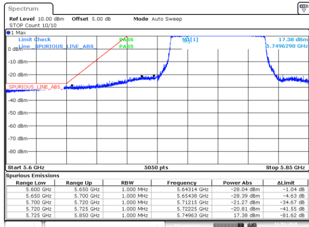
Date: 3 NOV 2020 18:48:52 BE-NR-LOW, SISO-A, 802.11ax80-HE0, Ch155
