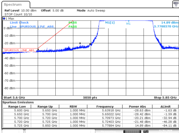
Date: 3 NOV 2020 19:04:43 BE-NR-LOW, SISO-A, 802.11ac80-VHT0, Ch155
