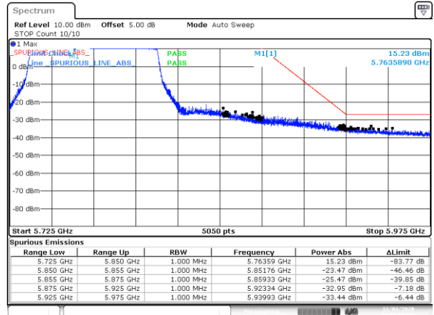
Date: 3 NOV 2020 19:05:50 BE-NR-HIGH, SISO-A, 802.11ac80-VHT0, Ch155
