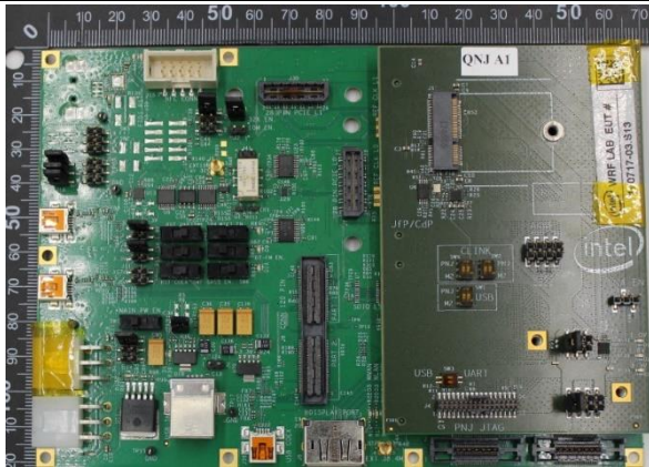
Socket front
