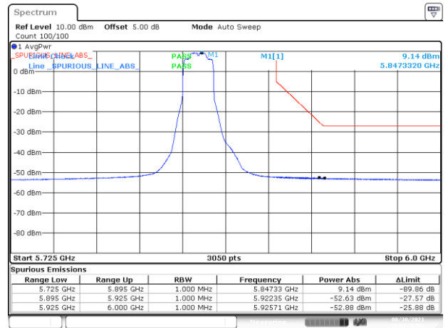
BE-NR-HIGH, MIMO-A, 802.11ax20-MCS0, Ch169
