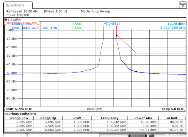
BE-NR-HIGH, SISO-B, 802.11ax20-MCS0, Ch177
