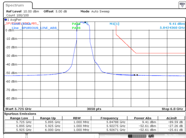
BE-NR-HIGH, MIMO-B, 802.11ax20-MCS0, Ch169
