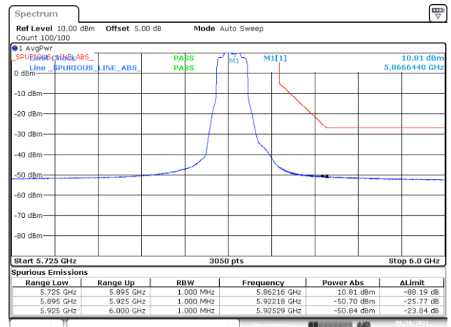
BE-NR-HIGH, SISO-A, 802.11ax20-MCS0, Ch173
